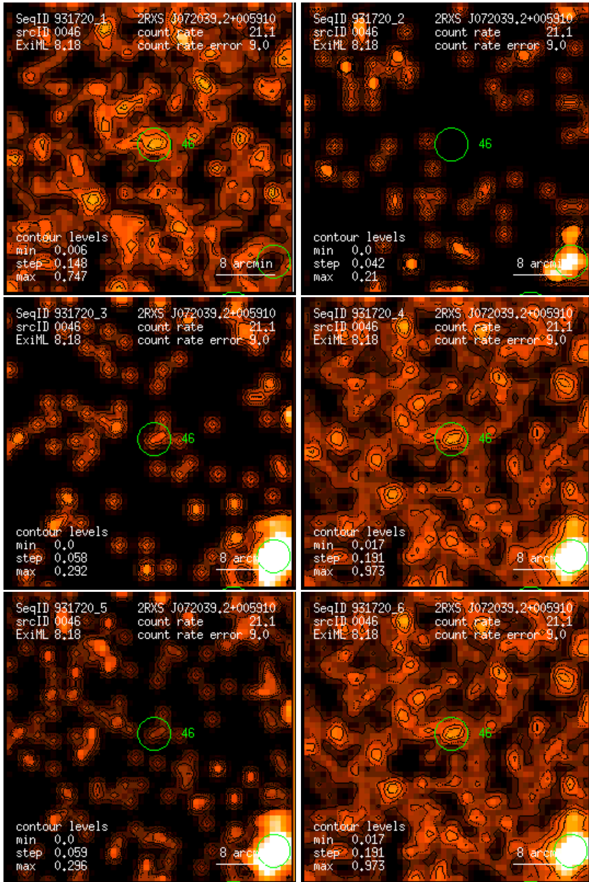
Figure 46: RASS 931720: detection 0046: band rate images, Gaussian filter: (1) PSPC channels 11 – 41, (2) 52 – 90, (3) 91 – 201, (4) 11 – 235, (5) 52 – 201, (6) 11 – 201. Broad band rates in counts/ks. Band rate contour levels in counts/ks/arcmin 2 .
