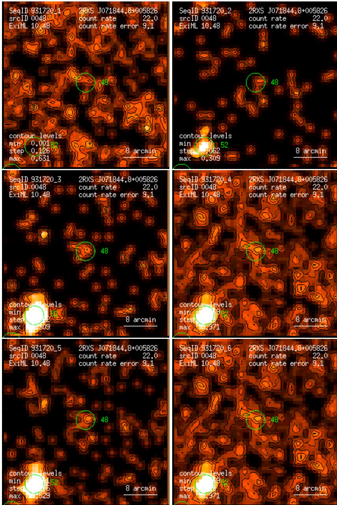
Figure 48: RASS 931720: detection 0048: band rate images, Gaussian filter: (1) PSPC channels 11 – 41, (2) 52 – 90, (3) 91 – 201, (4) 11 – 235, (5) 52 – 201, (6) 11 – 201. Broad band rates in counts/ks. Band rate contour levels in counts/ks/arcmin 2 .
