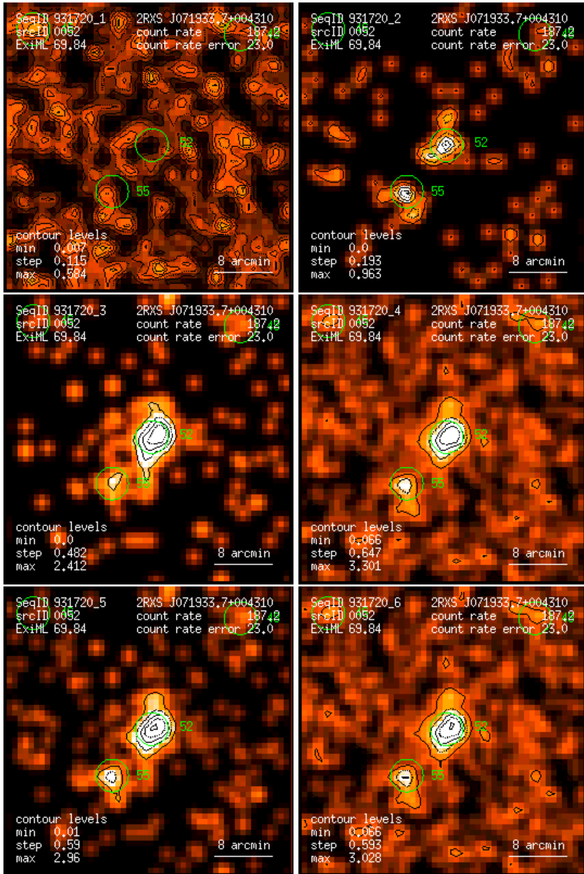
Figure 52: RASS 931720: detection 0052: band rate images, Gaussian filter: (1) PSPC channels 11 – 41, (2) 52 – 90, (3) 91 – 201, (4) 11 – 235, (5) 52 – 201, (6) 11 – 201. Broad band rates in counts/ks. Band rate contour levels in counts/ks/arcmin 2 .
