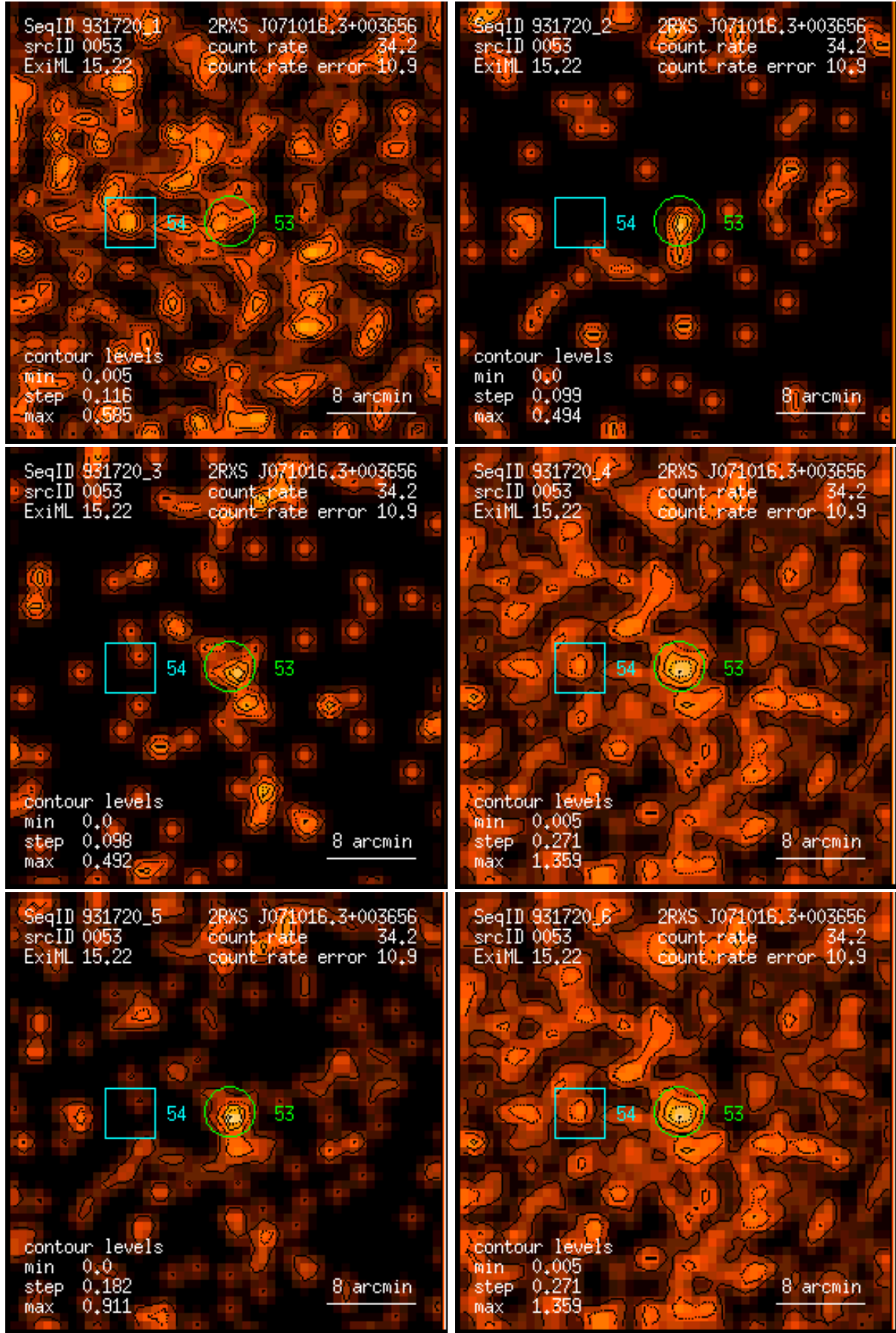
Figure 53: RASS 931720: detection 0053: band rate images, Gaussian filter: (1) PSPC channels 11 – 41, (2) 52 – 90, (3) 91 – 201, (4) 11 – 235, (5) 52 – 201, (6) 11 – 201. Broad band rates in counts/ks. Band rate contour levels in counts/ks/arcmin 2 .
