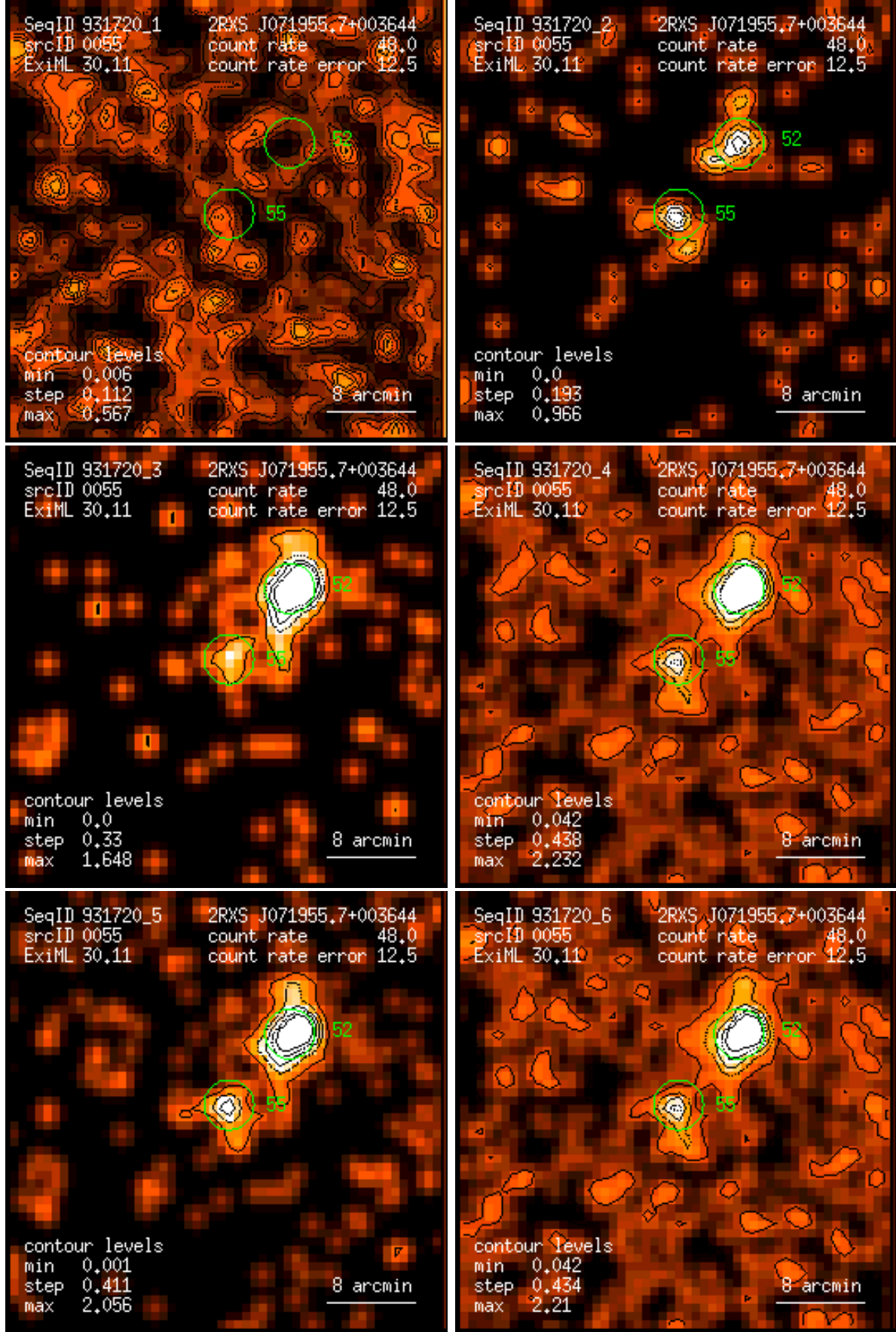
Figure 55: RASS 931720: detection 0055: band rate images, Gaussian filter: (1) PSPC channels 11 – 41, (2) 52 – 90, (3) 91 – 201, (4) 11 – 235, (5) 52 – 201, (6) 11 – 201. Broad band rates in counts/ks. Band rate contour levels in counts/ks/arcmin 2 .
