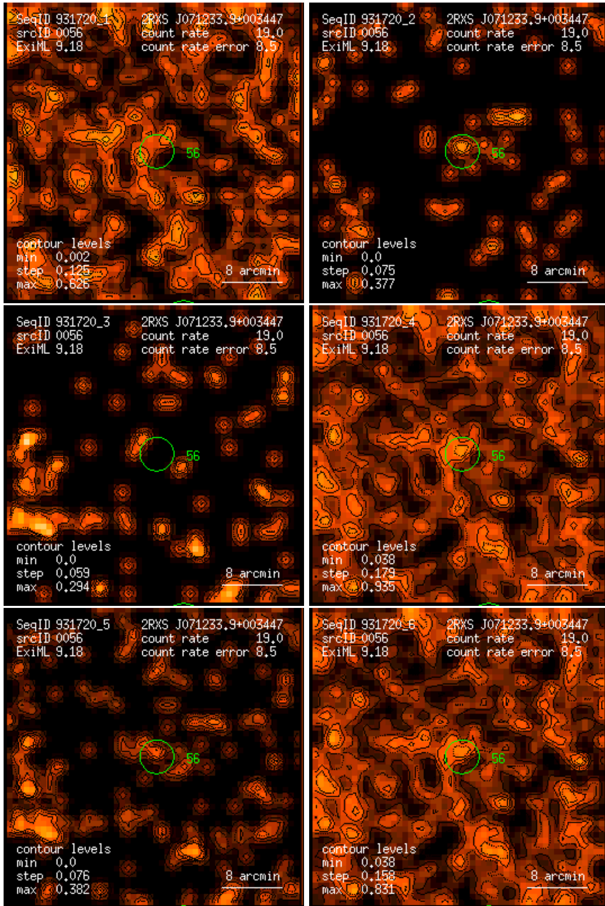
Figure 56: RASS 931720: detection 0056: band rate images, Gaussian filter: (1) PSPC channels 11 – 41, (2) 52 – 90, (3) 91 – 201, (4) 11 – 235, (5) 52 – 201, (6) 11 – 201. Broad band rates in counts/ks. Band rate contour levels in counts/ks/arcmin 2 .
