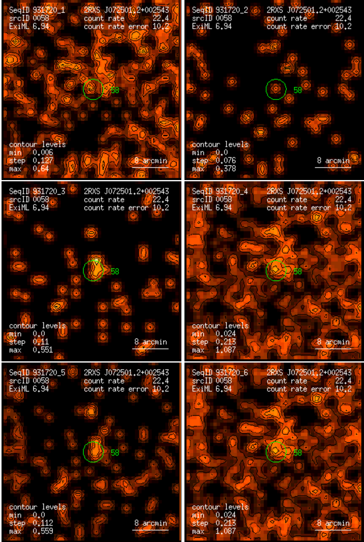
Figure 58: RASS 931720: detection 0058: band rate images, Gaussian filter: (1) PSPC channels 11 – 41, (2) 52 – 90, (3) 91 – 201, (4) 11 – 235, (5) 52 – 201, (6) 11 – 201. Broad band rates in counts/ks. Band rate contour levels in counts/ks/arcmin 2 .
