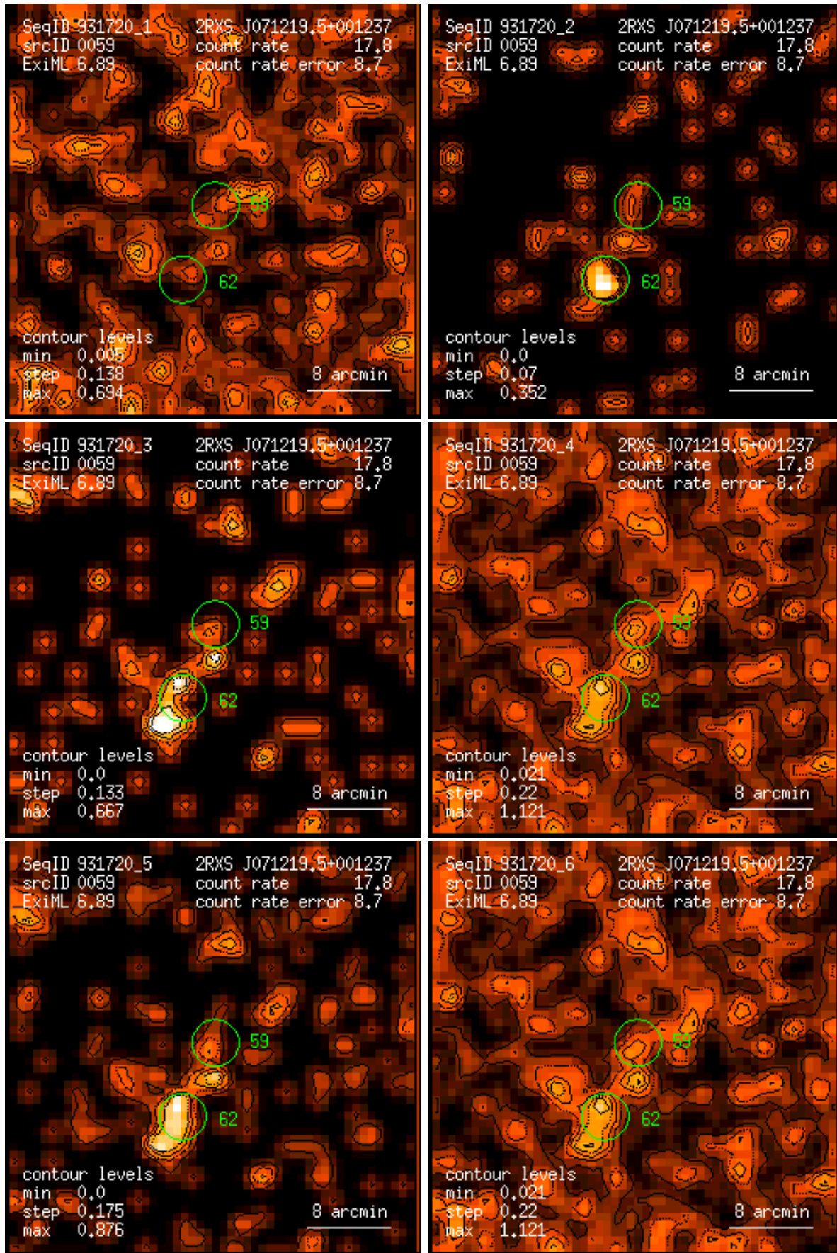
Figure 59: RASS 931720: detection 0059: band rate images, Gaussian filter: (1) PSPC channels 11 – 41, (2) 52 – 90, (3) 91 – 201, (4) 11 – 235, (5) 52 – 201, (6) 11 – 201. Broad band rates in counts/ks. Band rate contour levels in counts/ks/arcmin 2 .
