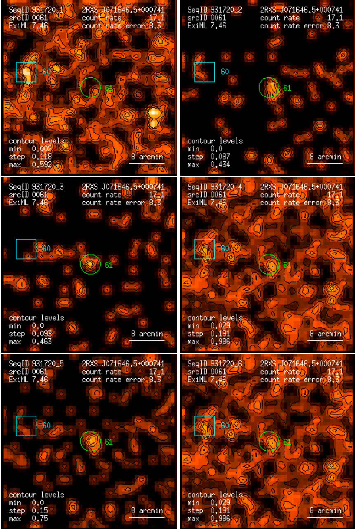
Figure 61: RASS 931720: detection 0061: band rate images, Gaussian filter: (1) PSPC channels 11 – 41, (2) 52 – 90, (3) 91 – 201, (4) 11 – 235, (5) 52 – 201, (6) 11 – 201. Broad band rates in counts/ks. Band rate contour levels in counts/ks/arcmin 2 .
