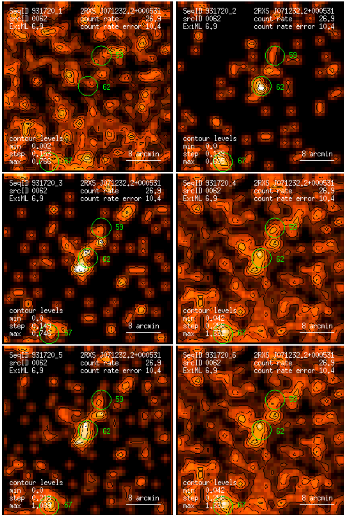
Figure 62: RASS 931720: detection 0062: band rate images, Gaussian filter: (1) PSPC channels 11 – 41, (2) 52 – 90, (3) 91 – 201, (4) 11 – 235, (5) 52 – 201, (6) 11 – 201. Broad band rates in counts/ks. Band rate contour levels in counts/ks/arcmin 2 .
