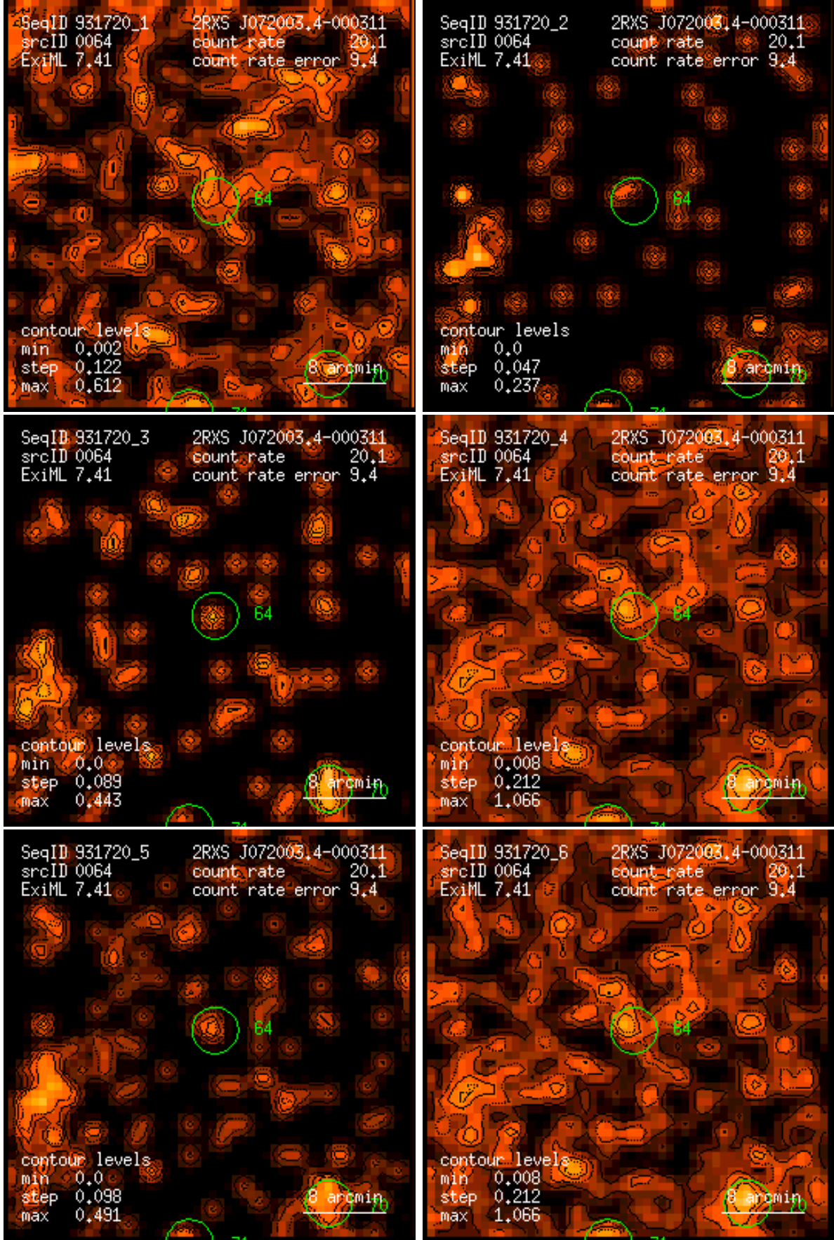
Figure 64: RASS 931720: detection 0064: band rate images, Gaussian filter: (1) PSPC channels 11 – 41, (2) 52 – 90, (3) 91 – 201, (4) 11 – 235, (5) 52 – 201, (6) 11 – 201. Broad band rates in counts/ks. Band rate contour levels in counts/ks/arcmin 2 .
