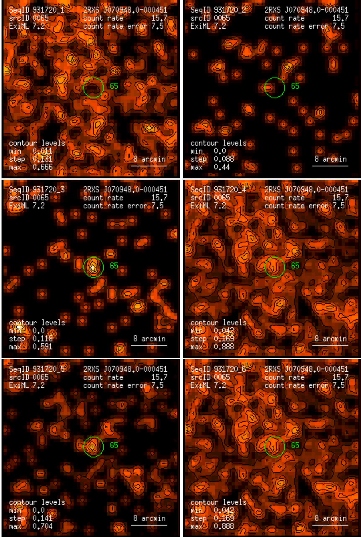
Figure 65: RASS 931720: detection 0065: band rate images, Gaussian filter: (1) PSPC channels 11 – 41, (2) 52 – 90, (3) 91 – 201, (4) 11 – 235, (5) 52 – 201, (6) 11 – 201. Broad band rates in counts/ks. Band rate contour levels in counts/ks/arcmin 2 .
