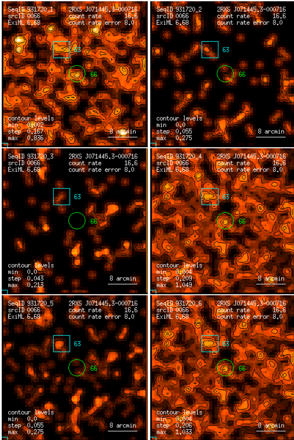
Figure 66: RASS 931720: detection 0066: band rate images, Gaussian filter: (1) PSPC channels 11 – 41, (2) 52 – 90, (3) 91 – 201, (4) 11 – 235, (5) 52 – 201, (6) 11 – 201. Broad band rates in counts/ks. Band rate contour levels in counts/ks/arcmin 2 .
