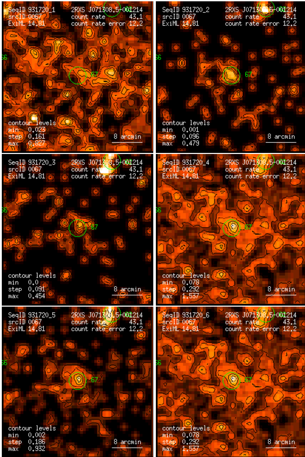
Figure 67: RASS 931720: detection 0067: band rate images, Gaussian filter: (1) PSPC channels 11 – 41, (2) 52 – 90, (3) 91 – 201, (4) 11 – 235, (5) 52 – 201, (6) 11 – 201. Broad band rates in counts/ks. Band rate contour levels in counts/ks/arcmin 2 .
