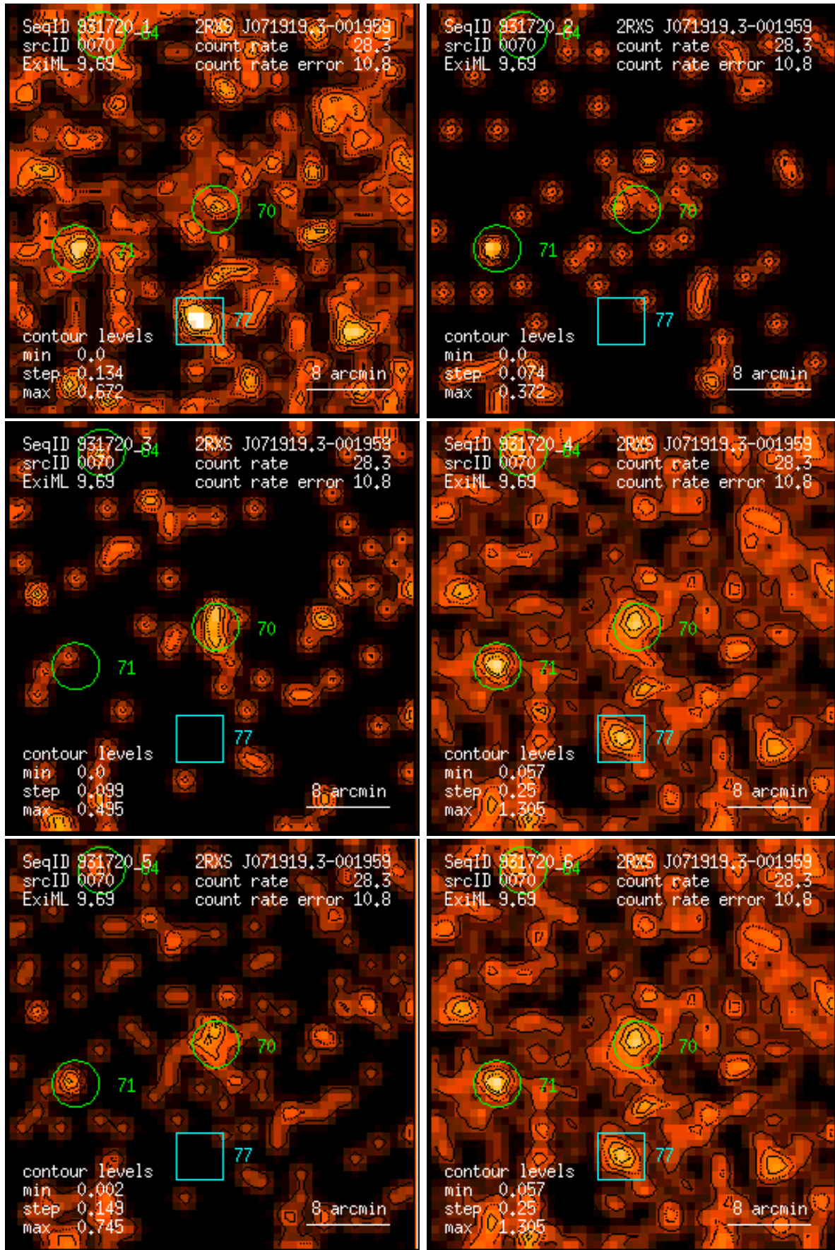
Figure 70: RASS 931720: detection 0070: band rate images, Gaussian filter: (1) PSPC channels 11 – 41, (2) 52 – 90, (3) 91 – 201, (4) 11 – 235, (5) 52 – 201, (6) 11 – 201. Broad band rates in counts/ks. Band rate contour levels in counts/ks/arcmin 2 .
