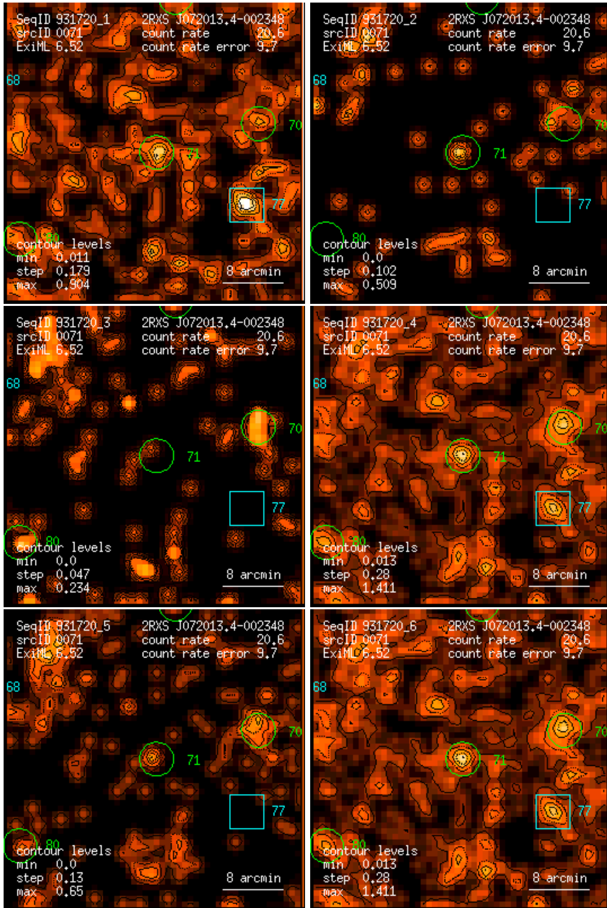
Figure 71: RASS 931720: detection 0071: band rate images, Gaussian filter: (1) PSPC channels 11 – 41, (2) 52 – 90, (3) 91 – 201, (4) 11 – 235, (5) 52 – 201, (6) 11 – 201. Broad band rates in counts/ks. Band rate contour levels in counts/ks/arcmin 2 .
