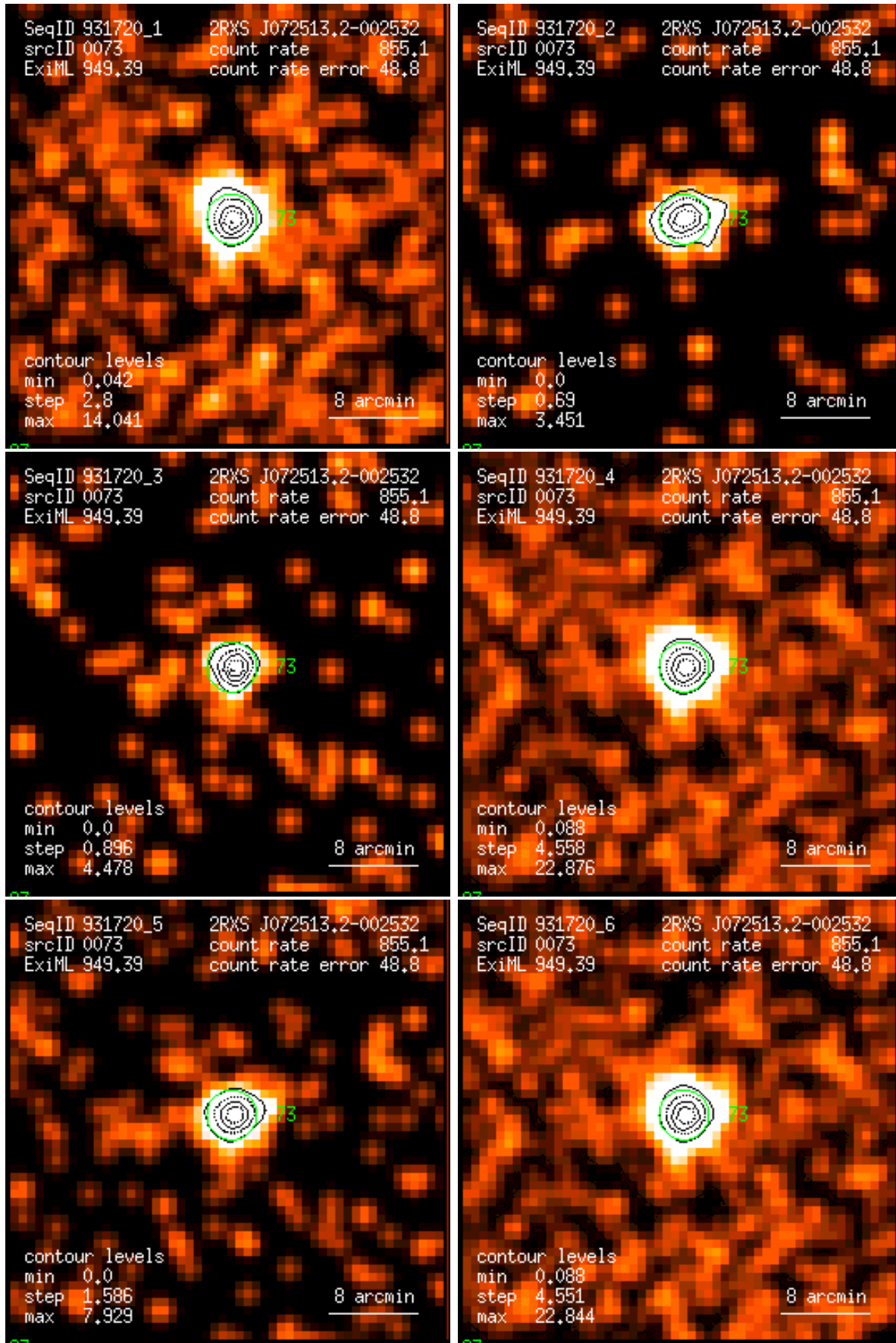
Figure 73: RASS 931720: detection 0073: band rate images, Gaussian filter: (1) PSPC channels 11 – 41, (2) 52 – 90, (3) 91 – 201, (4) 11 – 235, (5) 52 – 201, (6) 11 – 201. Broad band rates in counts/ks. Band rate contour levels in counts/ks/arcmin 2 .
