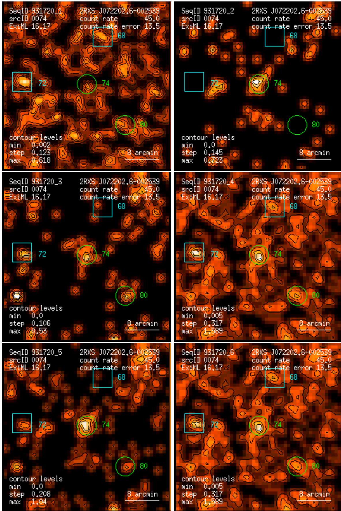
Figure 74: RASS 931720: detection 0074: band rate images, Gaussian filter: (1) PSPC channels 11 – 41, (2) 52 – 90, (3) 91 – 201, (4) 11 – 235, (5) 52 – 201, (6) 11 – 201. Broad band rates in counts/ks. Band rate contour levels in counts/ks/arcmin 2 .
