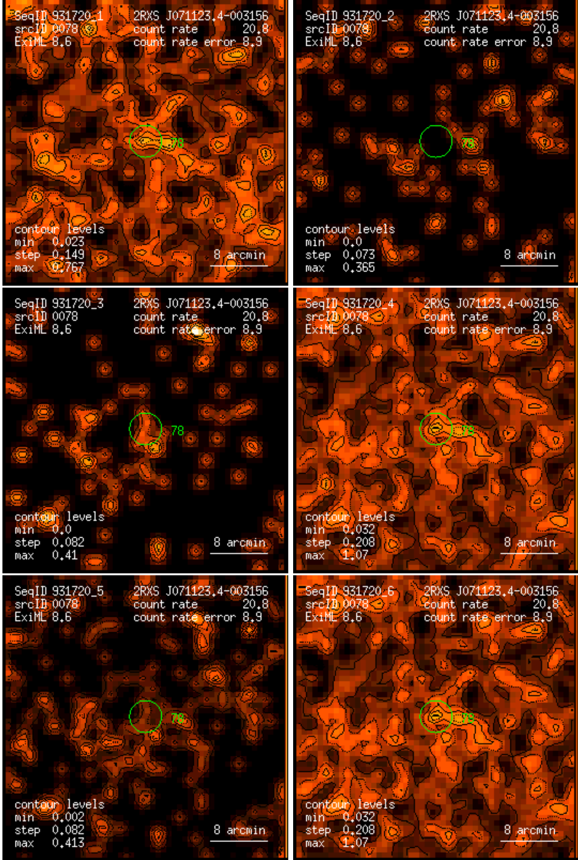
Figure 78: RASS 931720: detection 0078: band rate images, Gaussian filter: (1) PSPC channels 11 – 41, (2) 52 – 90, (3) 91 – 201, (4) 11 – 235, (5) 52 – 201, (6) 11 – 201. Broad band rates in counts/ks. Band rate contour levels in counts/ks/arcmin 2 .
