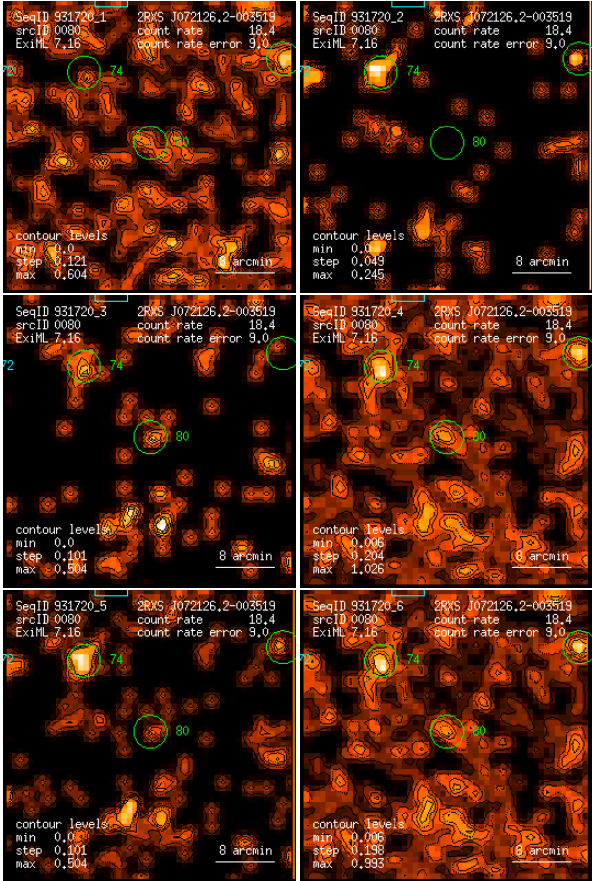
Figure 80: RASS 931720: detection 0080: band rate images, Gaussian filter: (1) PSPC channels 11 – 41, (2) 52 – 90, (3) 91 – 201, (4) 11 – 235, (5) 52 – 201, (6) 11 – 201. Broad band rates in counts/ks. Band rate contour levels in counts/ks/arcmin 2 .
