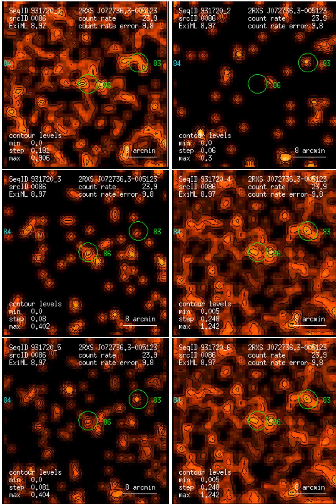
Figure 86: RASS 931720: detection 0086: band rate images, Gaussian filter: (1) PSPC channels 11 – 41, (2) 52 – 90, (3) 91 – 201, (4) 11 – 235, (5) 52 – 201, (6) 11 – 201. Broad band rates in counts/ks. Band rate contour levels in counts/ks/arcmin 2 .
