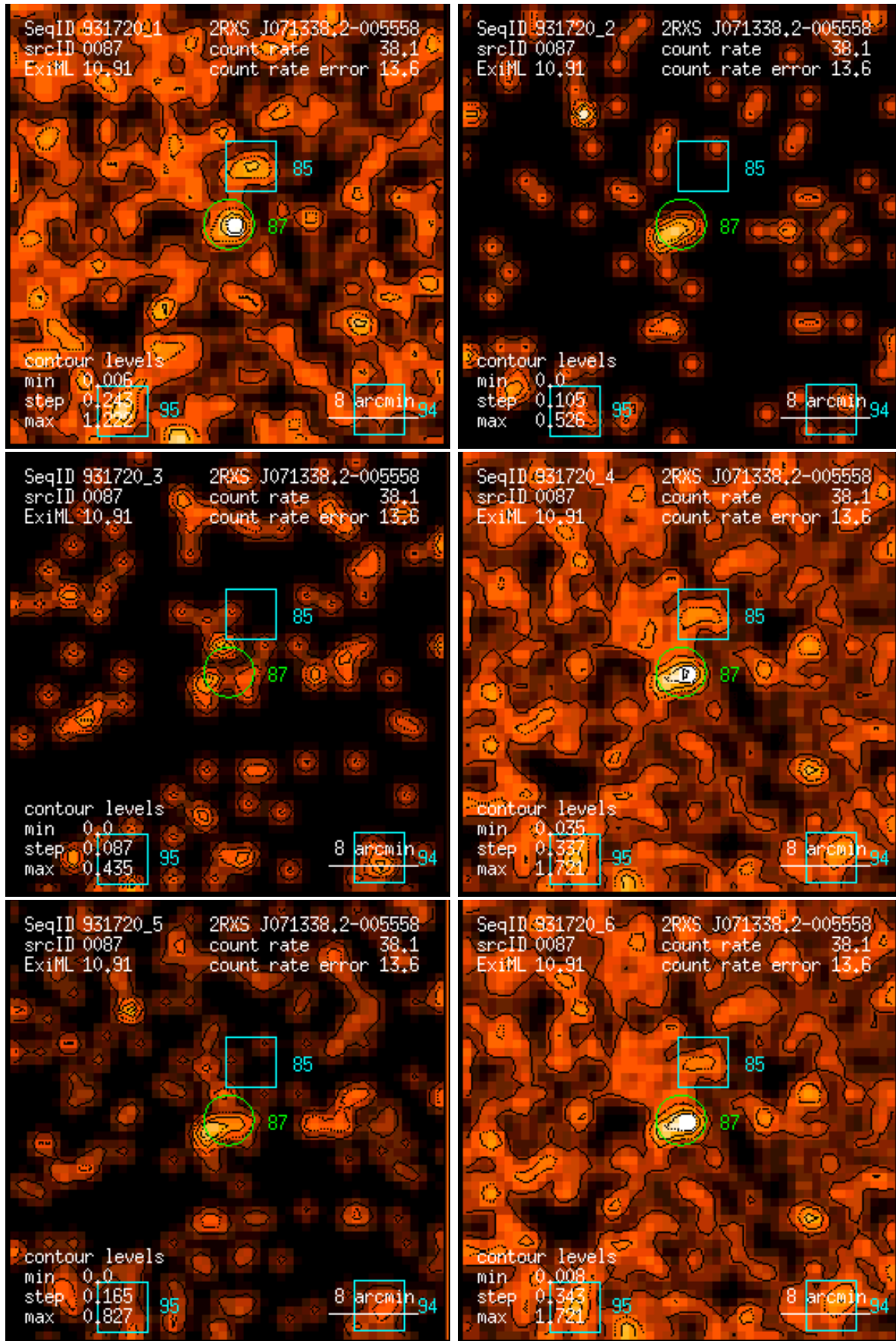
Figure 87: RASS 931720: detection 0087: band rate images, Gaussian filter: (1) PSPC channels 11 – 41, (2) 52 – 90, (3) 91 – 201, (4) 11 – 235, (5) 52 – 201, (6) 11 – 201. Broad band rates in counts/ks. Band rate contour levels in counts/ks/arcmin 2 .
