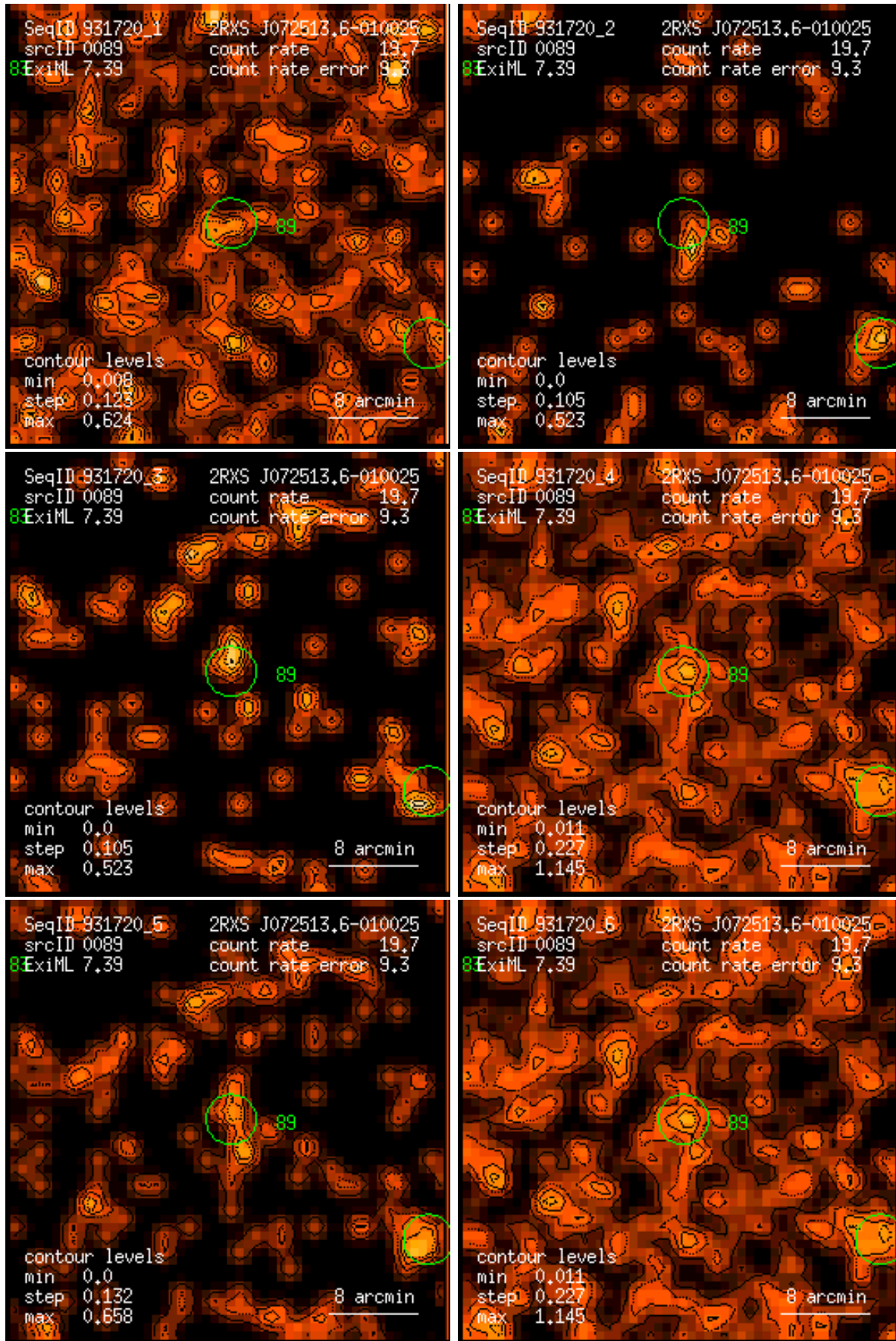
Figure 89: RASS 931720: detection 0089: band rate images, Gaussian filter: (1) PSPC channels 11 – 41, (2) 52 – 90, (3) 91 – 201, (4) 11 – 235, (5) 52 – 201, (6) 11 – 201. Broad band rates in counts/ks. Band rate contour levels in counts/ks/arcmin 2 .
