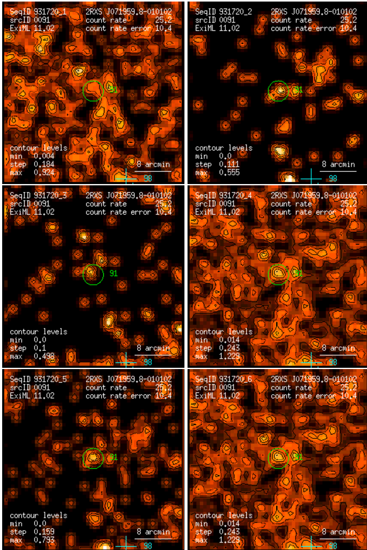
Figure 91: RASS 931720: detection 0091: band rate images, Gaussian filter: (1) PSPC channels 11 – 41, (2) 52 – 90, (3) 91 – 201, (4) 11 – 235, (5) 52 – 201, (6) 11 – 201. Broad band rates in counts/ks. Band rate contour levels in counts/ks/arcmin 2 .
