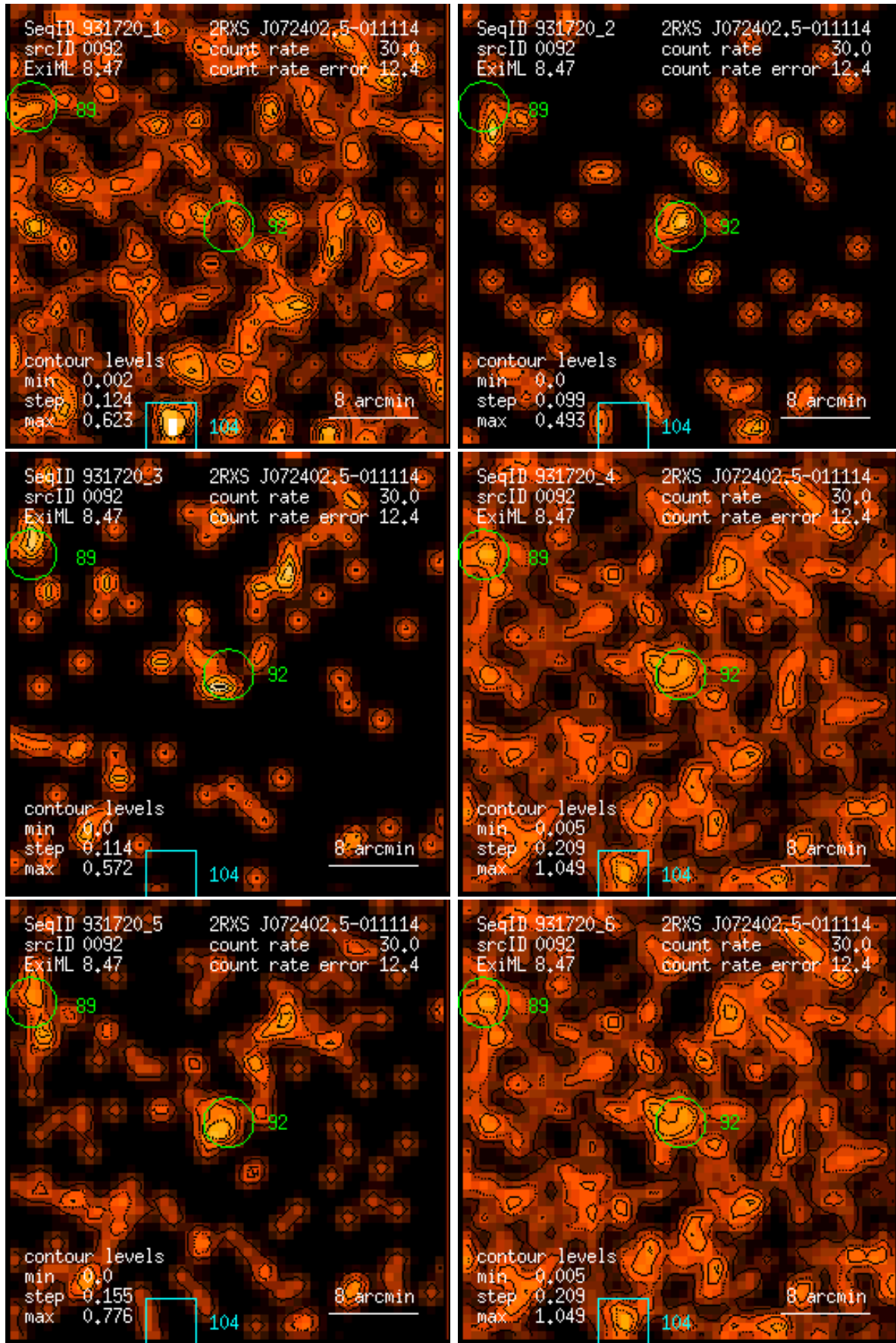
Figure 92: RASS 931720: detection 0092: band rate images, Gaussian filter: (1) PSPC channels 11 – 41, (2) 52 – 90, (3) 91 – 201, (4) 11 – 235, (5) 52 – 201, (6) 11 – 201. Broad band rates in counts/ks. Band rate contour levels in counts/ks/arcmin 2 .
