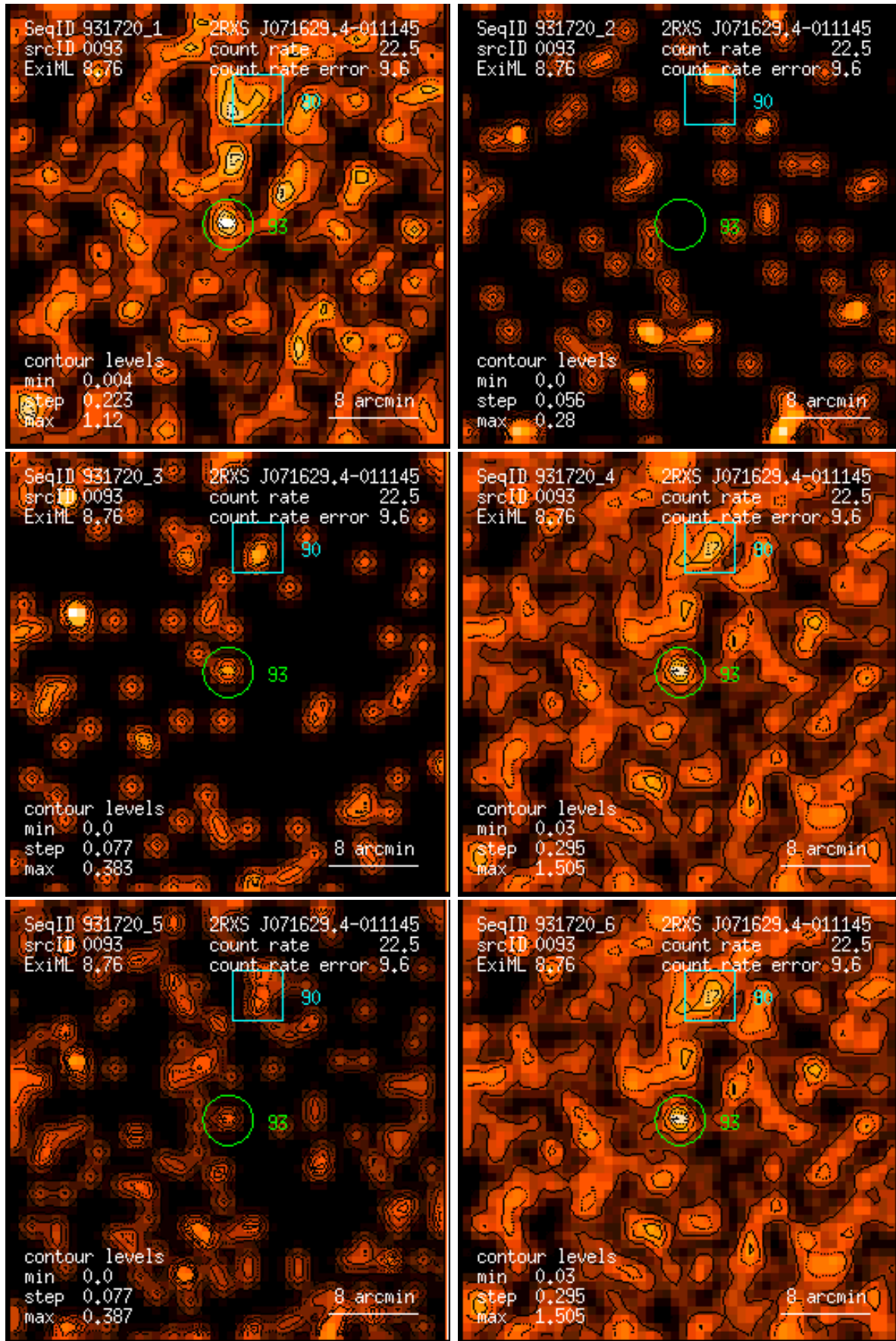
Figure 93: RASS 931720: detection 0093: band rate images, Gaussian filter: (1) PSPC channels 11 – 41, (2) 52 – 90, (3) 91 – 201, (4) 11 – 235, (5) 52 – 201, (6) 11 – 201. Broad band rates in counts/ks. Band rate contour levels in counts/ks/arcmin 2 .
