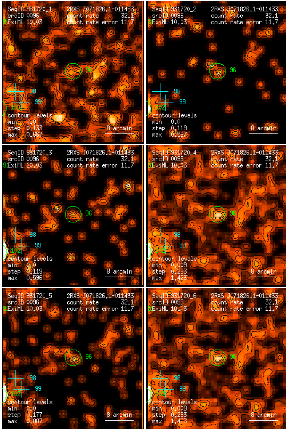
Figure 96: RASS 931720: detection 0096: band rate images, Gaussian filter: (1) PSPC channels 11 – 41, (2) 52 – 90, (3) 91 – 201, (4) 11 – 235, (5) 52 – 201, (6) 11 – 201. Broad band rates in counts/ks. Band rate contour levels in counts/ks/arcmin 2 .
