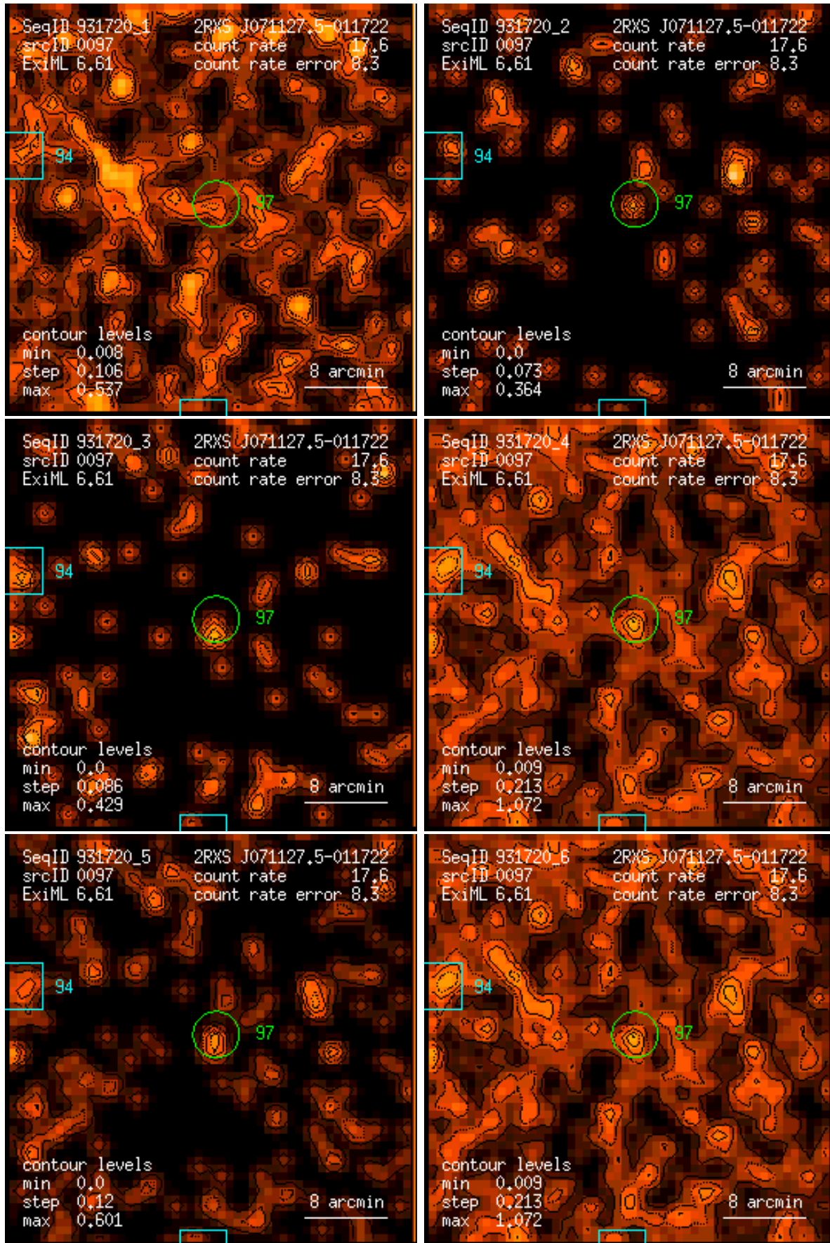
Figure 97: RASS 931720: detection 0097: band rate images, Gaussian filter: (1) PSPC channels 11 – 41, (2) 52 – 90, (3) 91 – 201, (4) 11 – 235, (5) 52 – 201, (6) 11 – 201. Broad band rates in counts/ks. Band rate contour levels in counts/ks/arcmin 2 .
