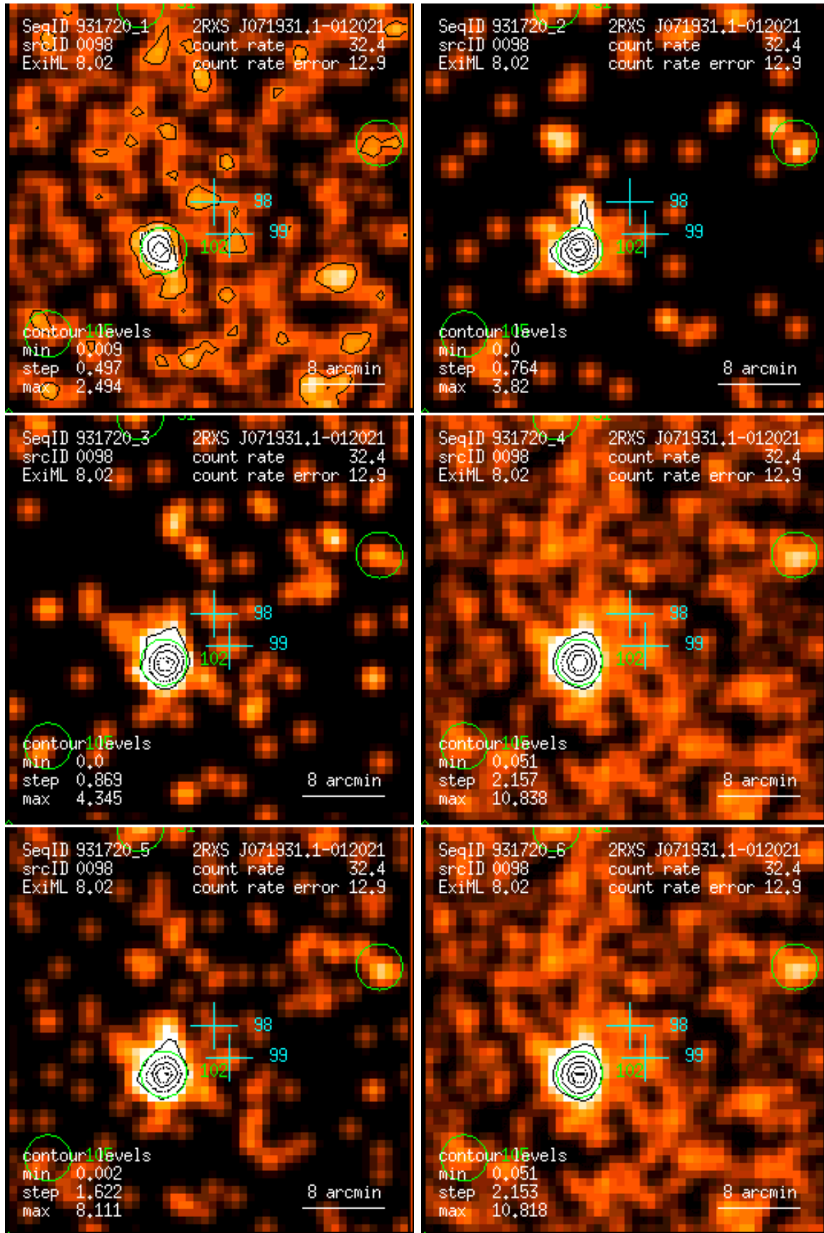
Figure 98: RASS 931720: detection 0098: band rate images, Gaussian filter: (1) PSPC channels 11 – 41, (2) 52 – 90, (3) 91 – 201, (4) 11 – 235, (5) 52 – 201, (6) 11 – 201. Broad band rates in counts/ks. Band rate contour levels in counts/ks/arcmin 2 .
