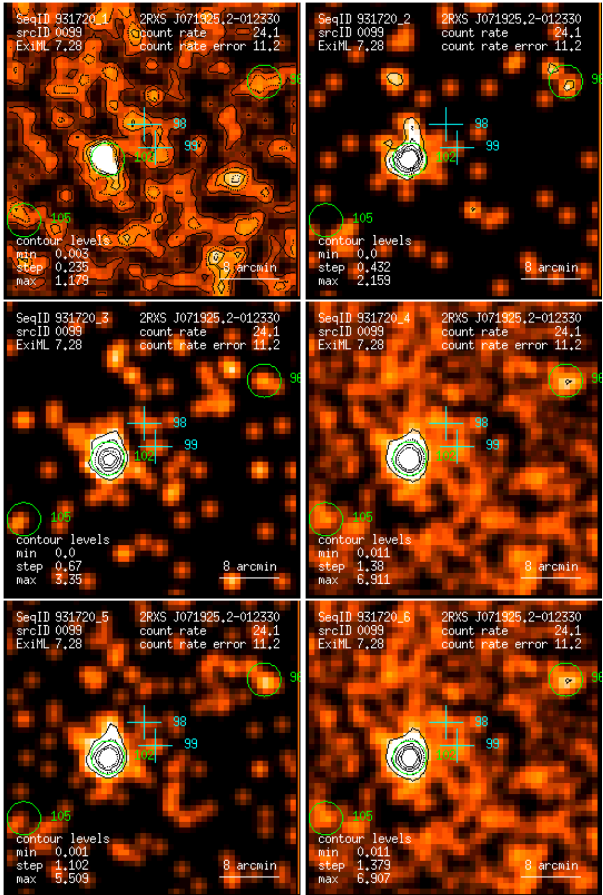
Figure 99: RASS 931720: detection 0099: band rate images, Gaussian filter: (1) PSPC channels 11 – 41, (2) 52 – 90, (3) 91 – 201, (4) 11 – 235, (5) 52 – 201, (6) 11 – 201. Broad band rates in counts/ks. Band rate contour levels in counts/ks/arcmin 2 .
