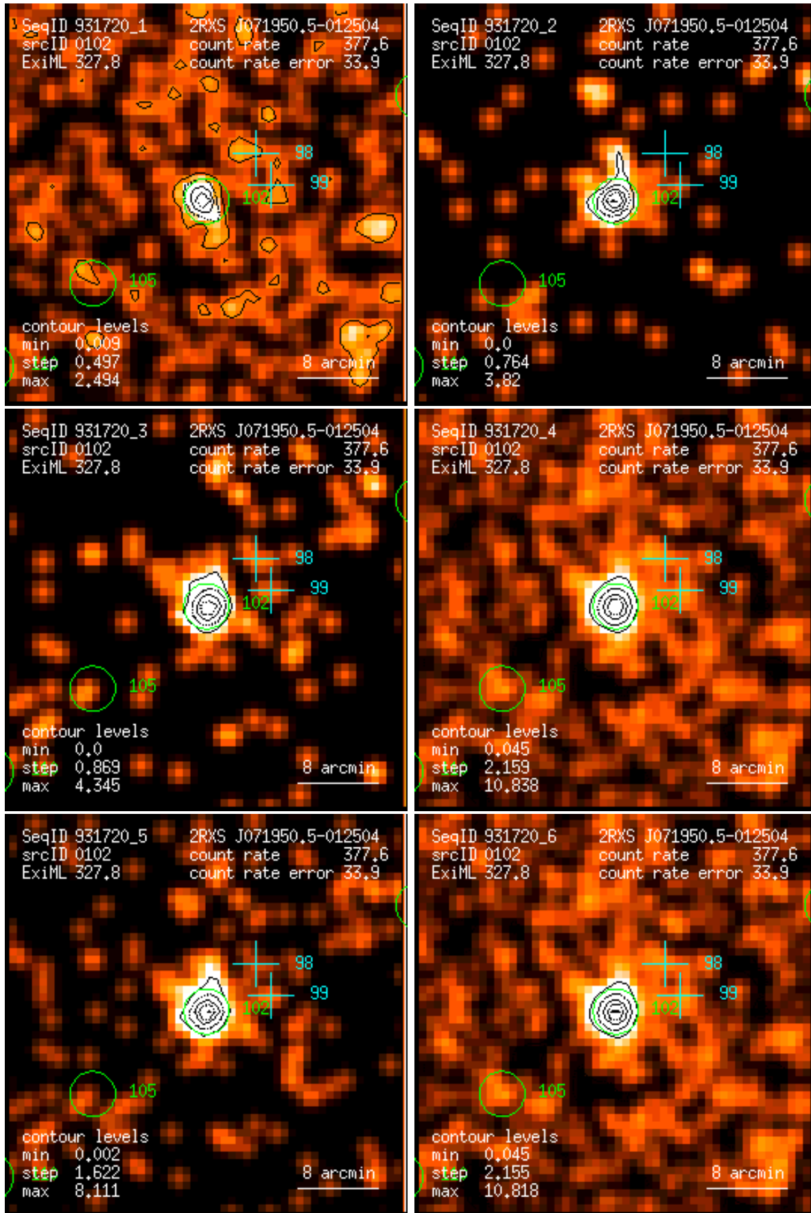
Figure 102: RASS 931720: detection 0102: band rate images, Gaussian filter: (1) PSPC channels 11 – 41, (2) 52 – 90, (3) 91 – 201, (4) 11 – 235, (5) 52 – 201, (6) 11 – 201. Broad band rates in counts/ks. Band rate contour levels in counts/ks/arcmin 2 .
