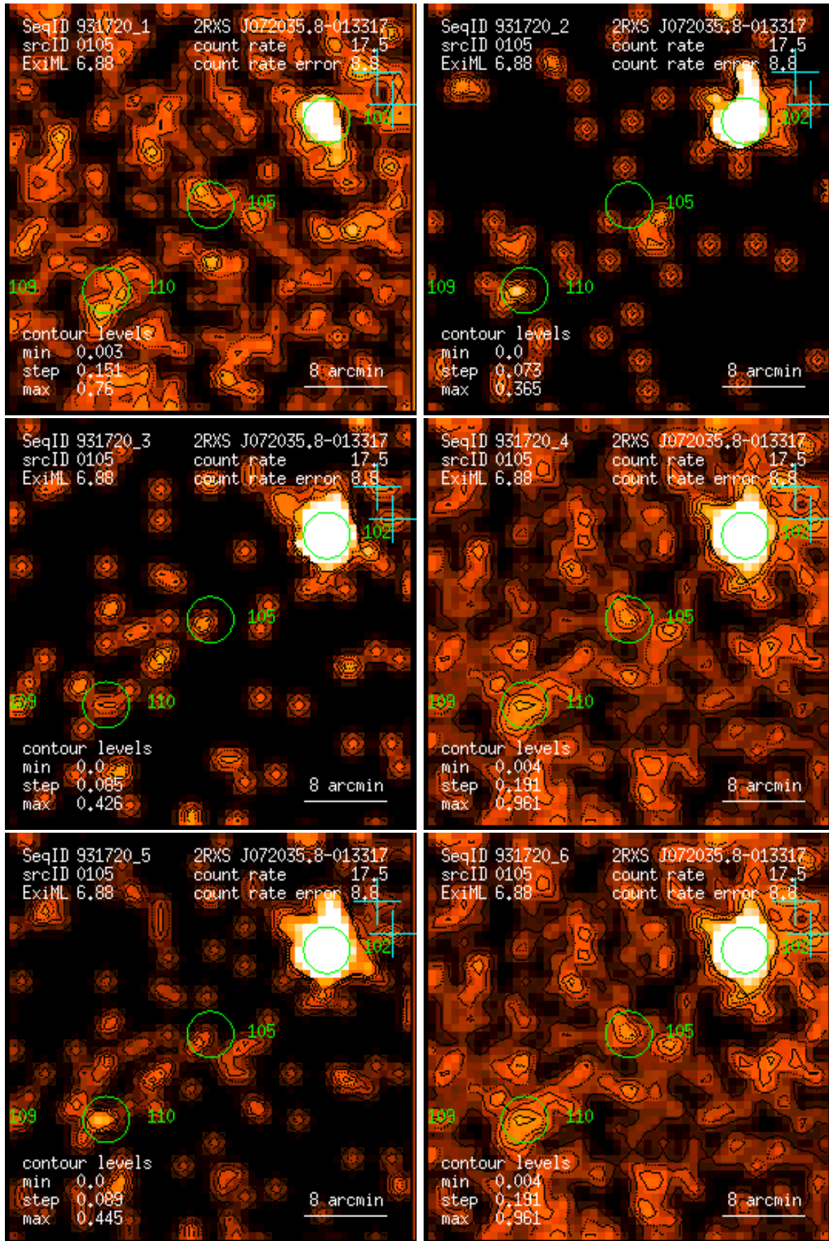
Figure 105: RASS 931720: detection 0105: band rate images, Gaussian filter: (1) PSPC channels 11 – 41, (2) 52 – 90, (3) 91 – 201, (4) 11 – 235, (5) 52 – 201, (6) 11 – 201. Broad band rates in counts/ks. Band rate contour levels in counts/ks/arcmin 2 .
