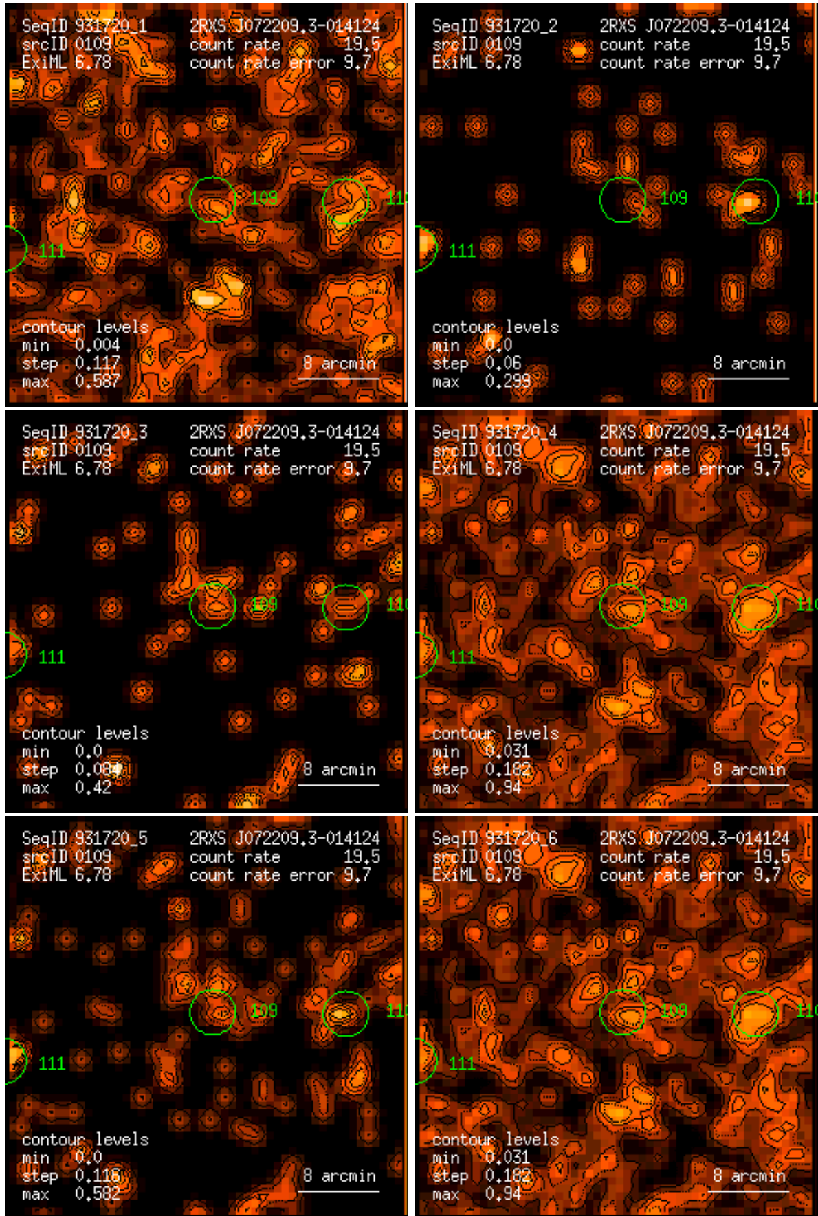
Figure 109: RASS 931720: detection 0109: band rate images, Gaussian filter: (1) PSPC channels 11 – 41, (2) 52 – 90, (3) 91 – 201, (4) 11 – 235, (5) 52 – 201, (6) 11 – 201. Broad band rates in counts/ks. Band rate contour levels in counts/ks/arcmin 2 .
