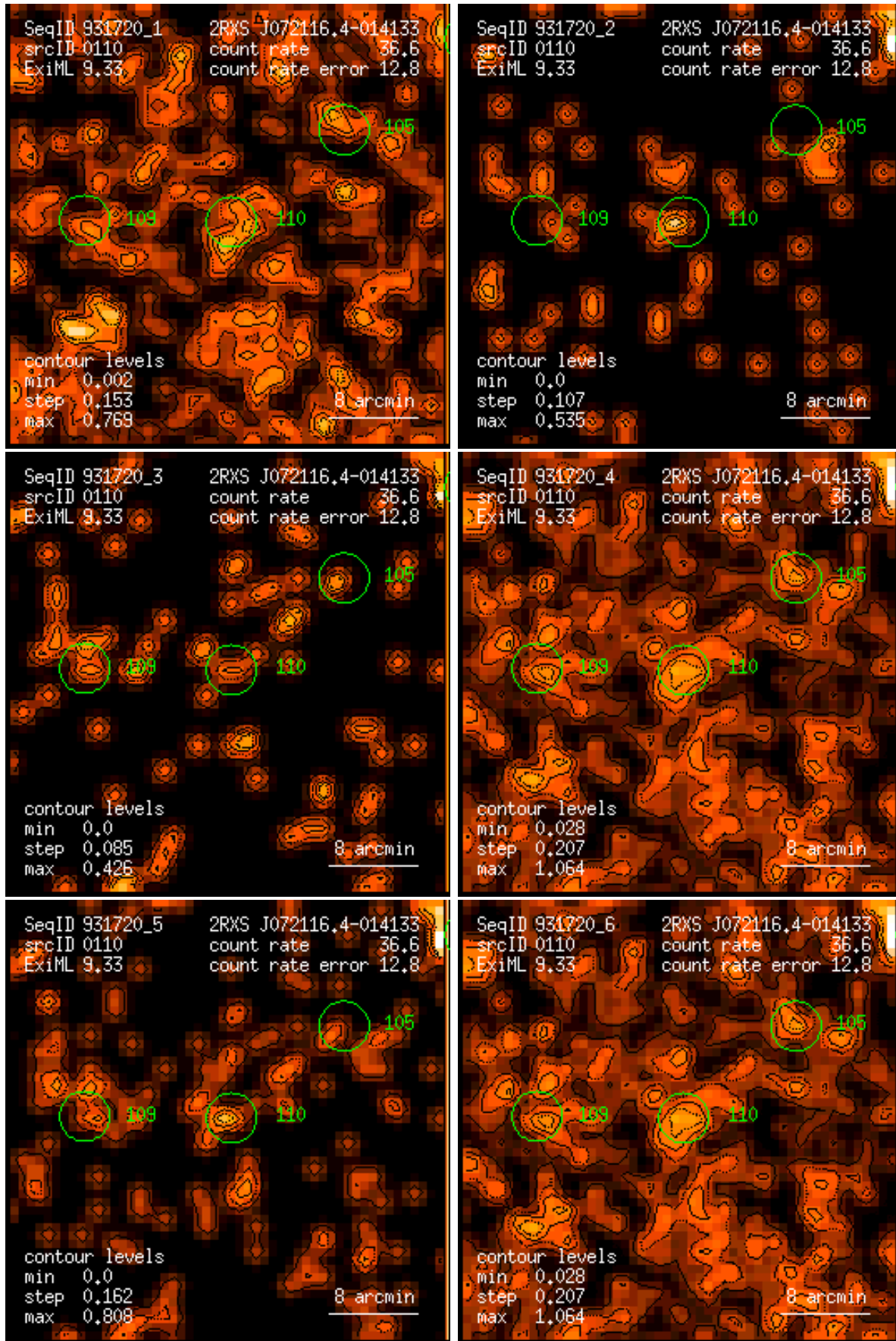
Figure 110: RASS 931720: detection 0110: band rate images, Gaussian filter: (1) PSPC channels 11 – 41, (2) 52 – 90, (3) 91 – 201, (4) 11 – 235, (5) 52 – 201, (6) 11 – 201. Broad band rates in counts/ks. Band rate contour levels in counts/ks/arcmin 2 .
