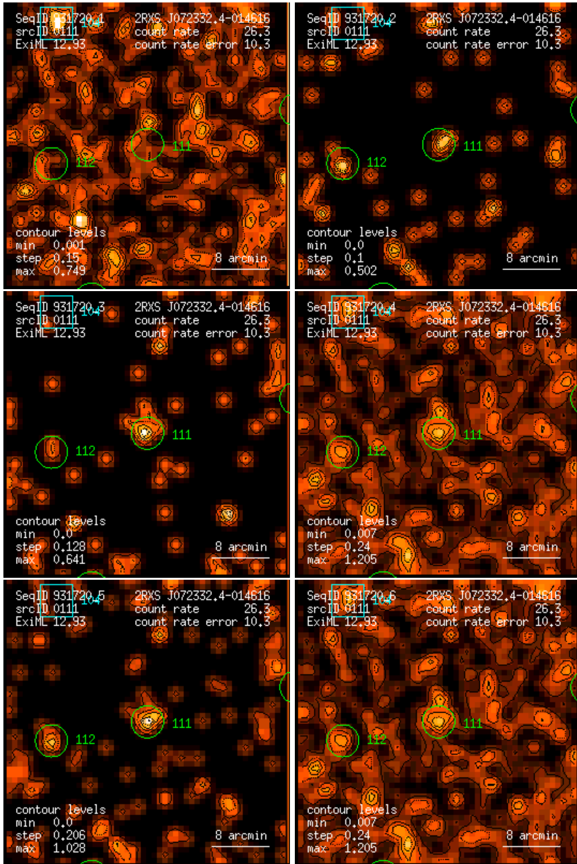
Figure 111: RASS 931720: detection 0111: band rate images, Gaussian filter: (1) PSPC channels 11 – 41, (2) 52 – 90, (3) 91 – 201, (4) 11 – 235, (5) 52 – 201, (6) 11 – 201. Broad band rates in counts/ks. Band rate contour levels in counts/ks/arcmin 2 .
