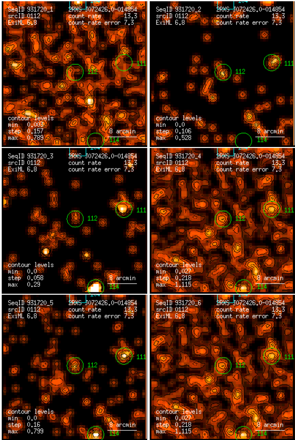
Figure 112: RASS 931720: detection 0112: band rate images, Gaussian filter: (1) PSPC channels 11 – 41, (2) 52 – 90, (3) 91 – 201, (4) 11 – 235, (5) 52 – 201, (6) 11 – 201. Broad band rates in counts/ks. Band rate contour levels in counts/ks/arcmin 2 .
