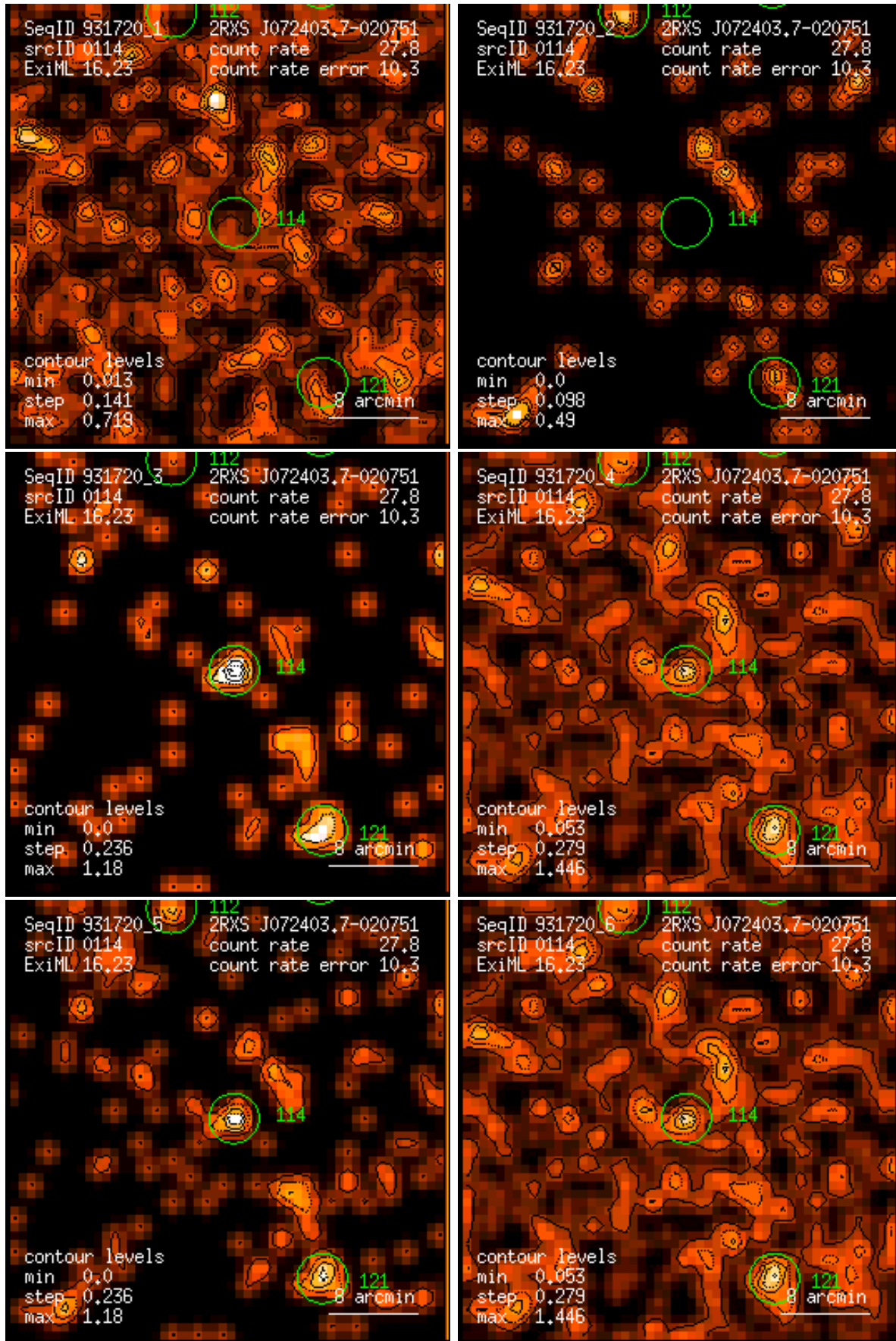
Figure 114: RASS 931720: detection 0114: band rate images, Gaussian filter: (1) PSPC channels 11 – 41, (2) 52 – 90, (3) 91 – 201, (4) 11 – 235, (5) 52 – 201, (6) 11 – 201. Broad band rates in counts/ks. Band rate contour levels in counts/ks/arcmin 2 .
