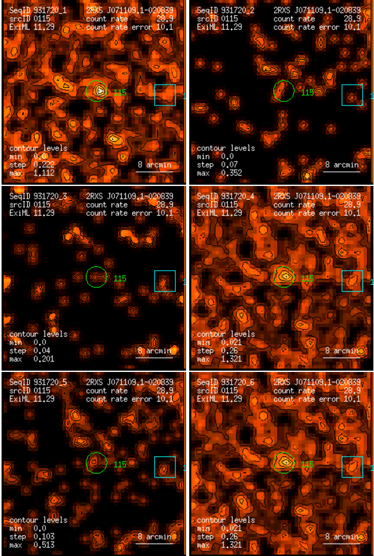
Figure 115: RASS 931720: detection 0115: band rate images, Gaussian filter: (1) PSPC channels 11 – 41, (2) 52 – 90, (3) 91 – 201, (4) 11 – 235, (5) 52 – 201, (6) 11 – 201. Broad band rates in counts/ks. Band rate contour levels in counts/ks/arcmin 2 .
