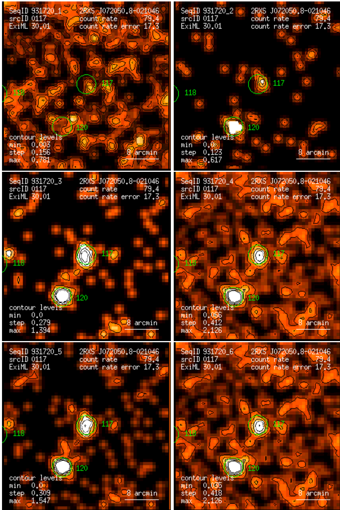
Figure 117: RASS 931720: detection 0117: band rate images, Gaussian filter: (1) PSPC channels 11 – 41, (2) 52 – 90, (3) 91 – 201, (4) 11 – 235, (5) 52 – 201, (6) 11 – 201. Broad band rates in counts/ks. Band rate contour levels in counts/ks/arcmin 2 .
