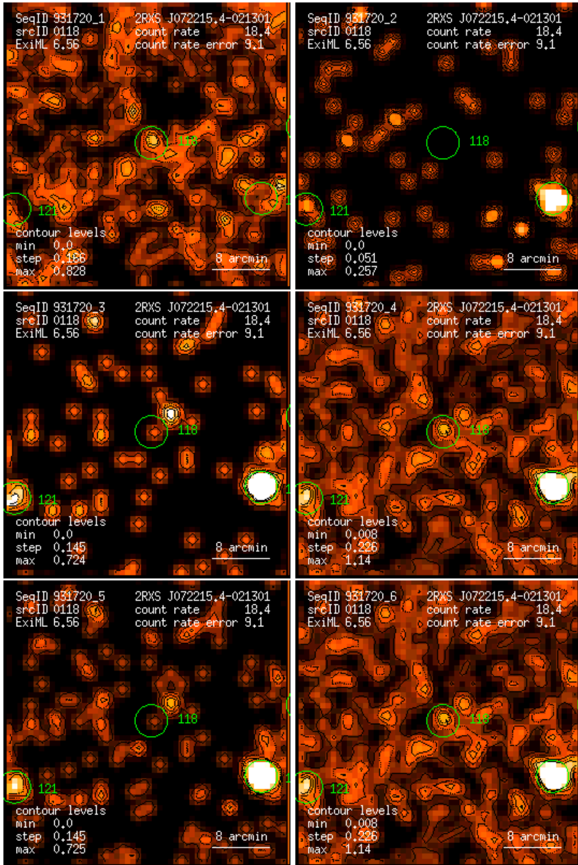
Figure 118: RASS 931720: detection 0118: band rate images, Gaussian filter: (1) PSPC channels 11 – 41, (2) 52 – 90, (3) 91 – 201, (4) 11 – 235, (5) 52 – 201, (6) 11 – 201. Broad band rates in counts/ks. Band rate contour levels in counts/ks/arcmin 2 .
