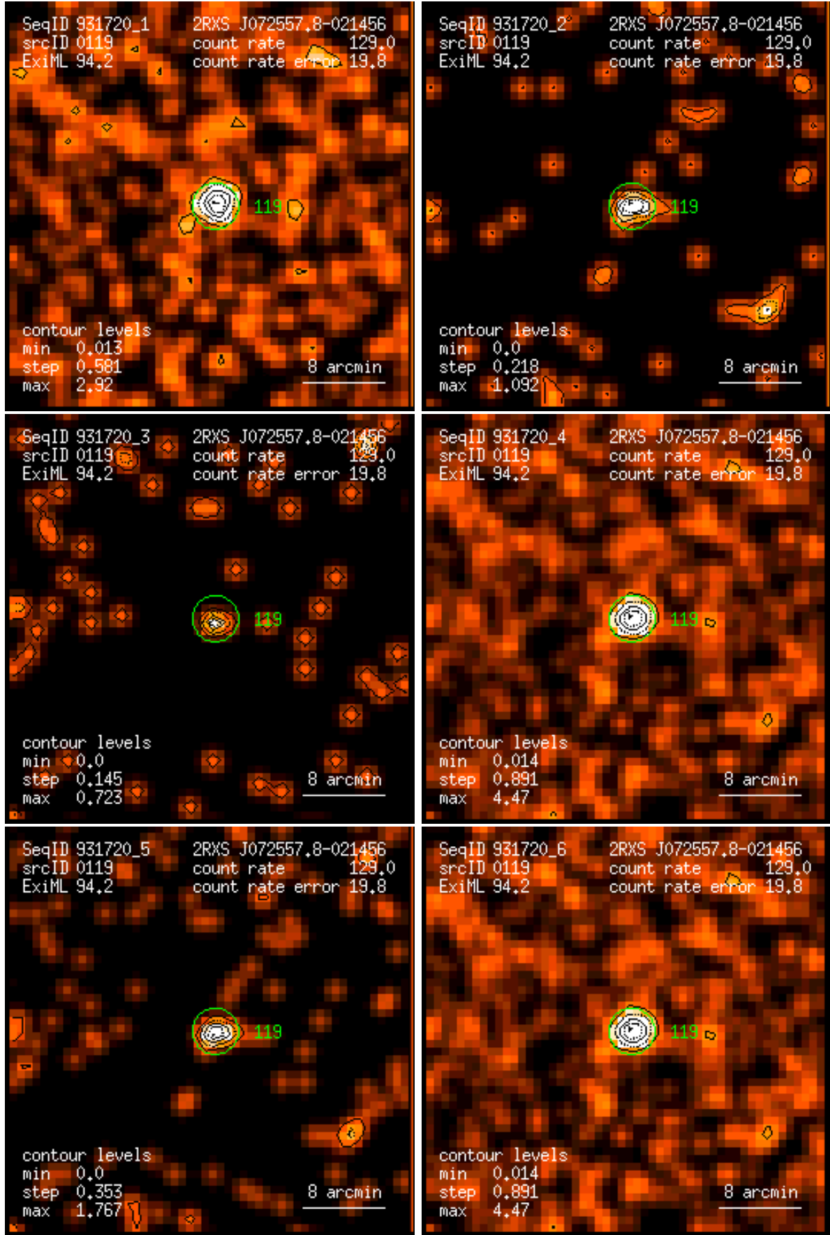
Figure 119: RASS 931720: detection 0119: band rate images, Gaussian filter: (1) PSPC channels 11 – 41, (2) 52 – 90, (3) 91 – 201, (4) 11 – 235, (5) 52 – 201, (6) 11 – 201. Broad band rates in counts/ks. Band rate contour levels in counts/ks/arcmin 2 .
