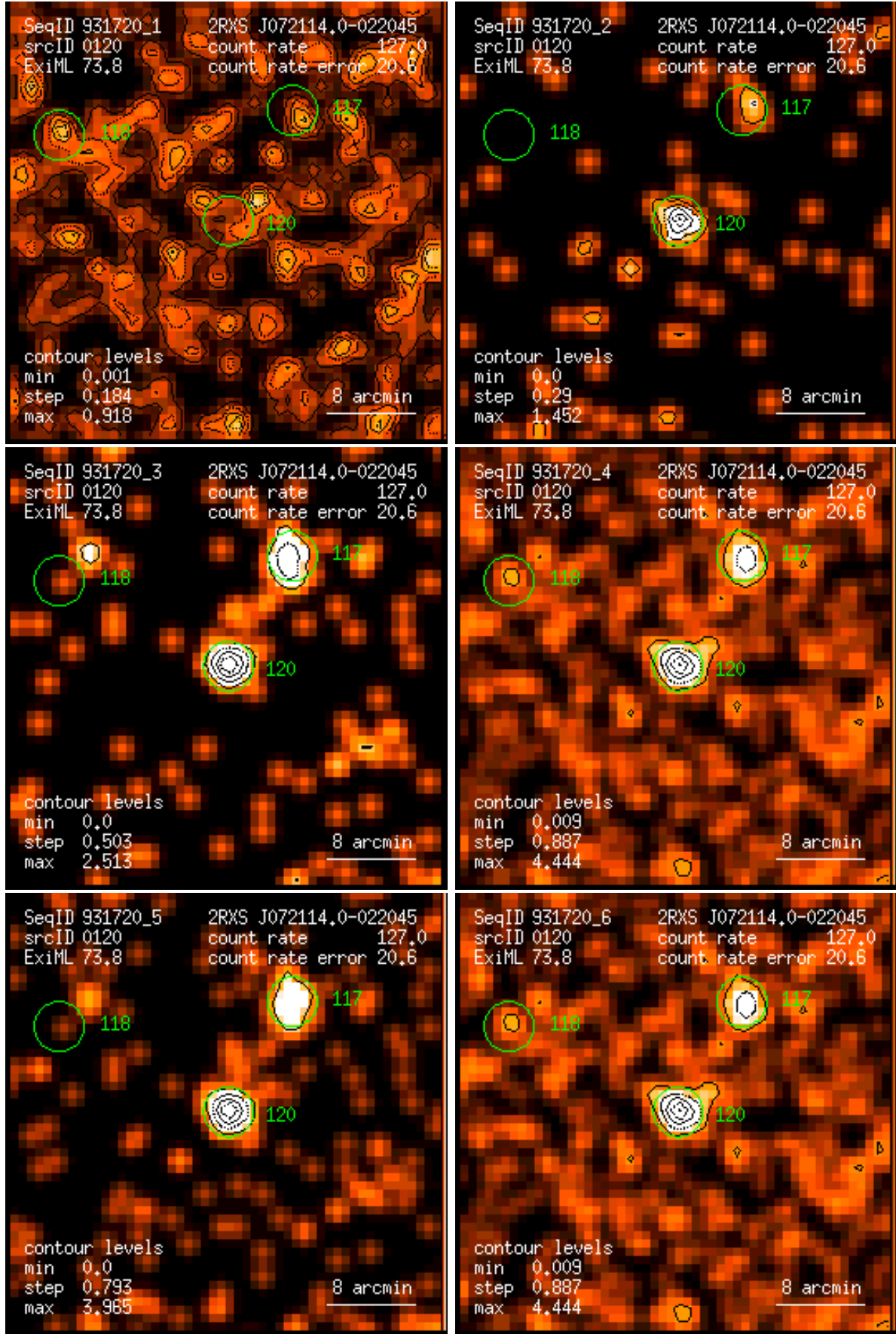
Figure 120: RASS 931720: detection 0120: band rate images, Gaussian filter: (1) PSPC channels 11 – 41, (2) 52 – 90, (3) 91 – 201, (4) 11 – 235, (5) 52 – 201, (6) 11 – 201. Broad band rates in counts/ks. Band rate contour levels in counts/ks/arcmin 2 .
