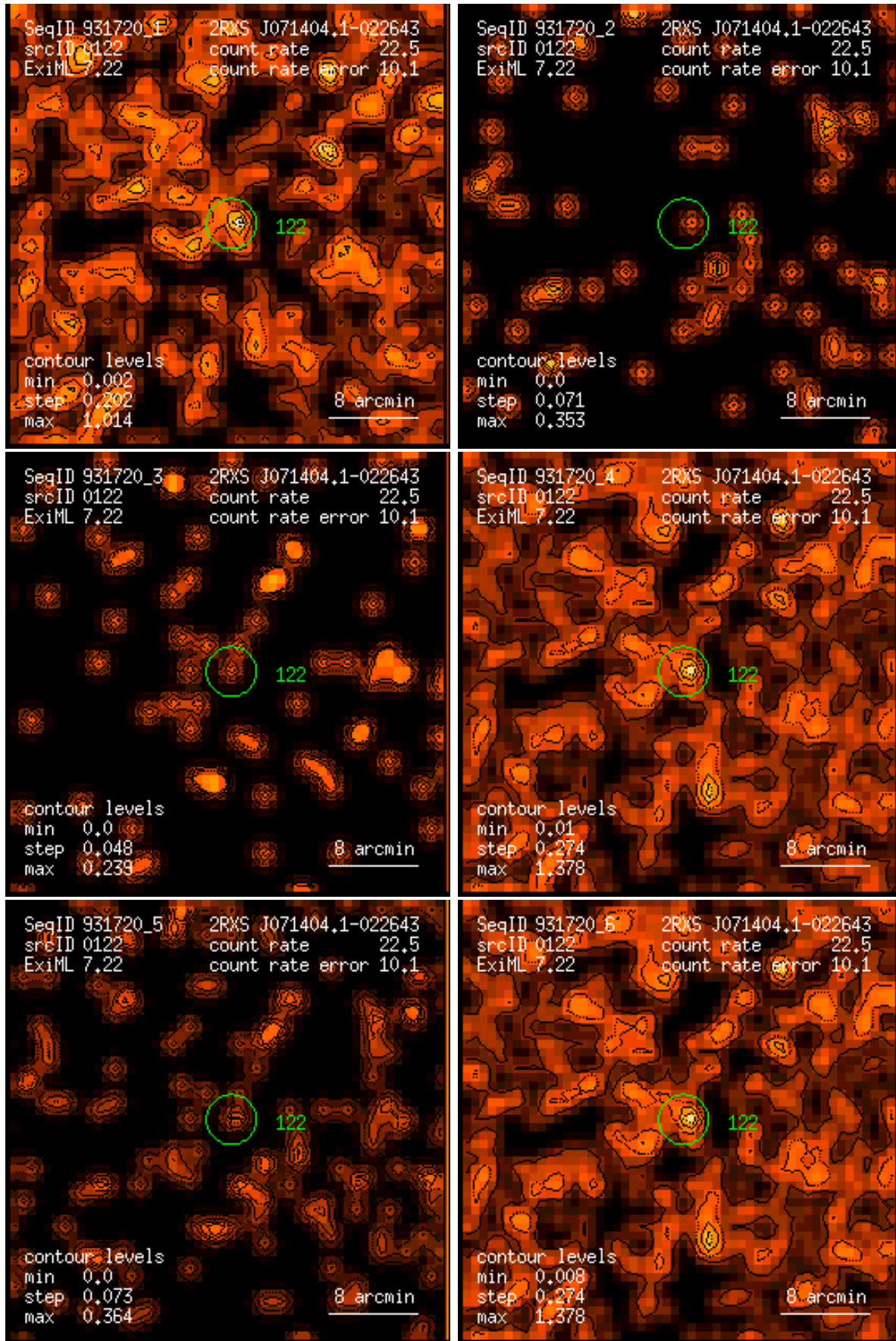
Figure 122: RASS 931720: detection 0122: band rate images, Gaussian filter: (1) PSPC channels 11 – 41, (2) 52 – 90, (3) 91 – 201, (4) 11 – 235, (5) 52 – 201, (6) 11 – 201. Broad band rates in counts/ks. Band rate contour levels in counts/ks/arcmin 2 .
