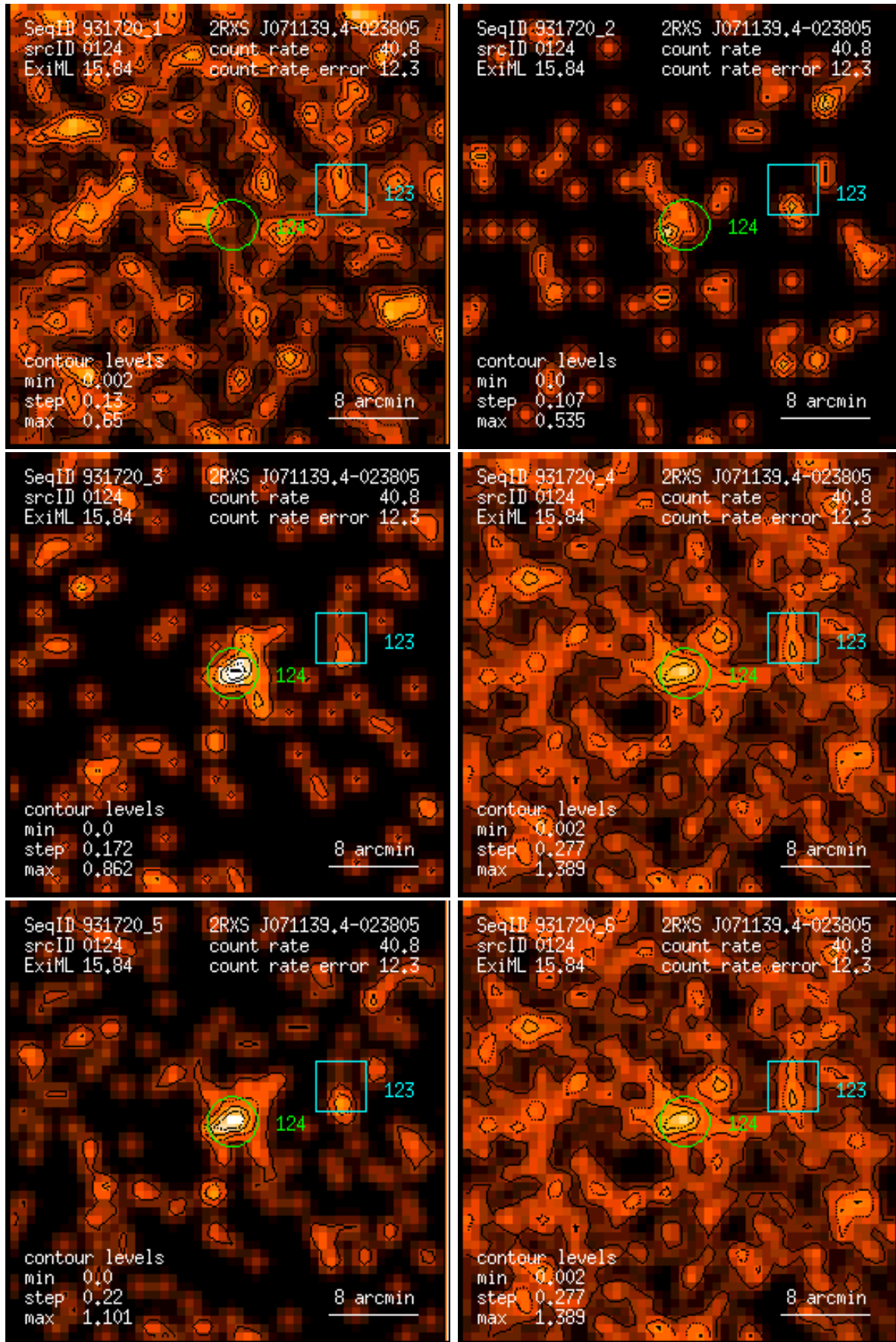
Figure 124: RASS 931720: detection 0124: band rate images, Gaussian filter: (1) PSPC channels 11 – 41, (2) 52 – 90, (3) 91 – 201, (4) 11 – 235, (5) 52 – 201, (6) 11 – 201. Broad band rates in counts/ks. Band rate contour levels in counts/ks/arcmin 2 .
