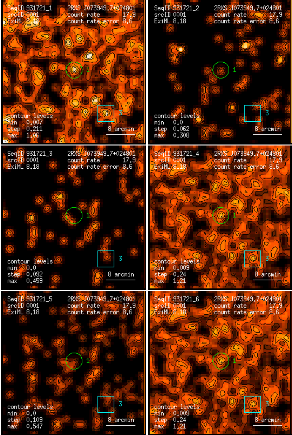
Figure 1: RASS 931721: detection 0001: band rate images, Gaussian filter: (1) PSPC channels 11 – 41, (2) 52 – 90, (3) 91 – 201, (4) 11 – 235, (5) 52 – 201, (6) 11 – 201. Broad band rates in counts/ks. Band rate contour levels in counts/ks/arcmin 2 .
