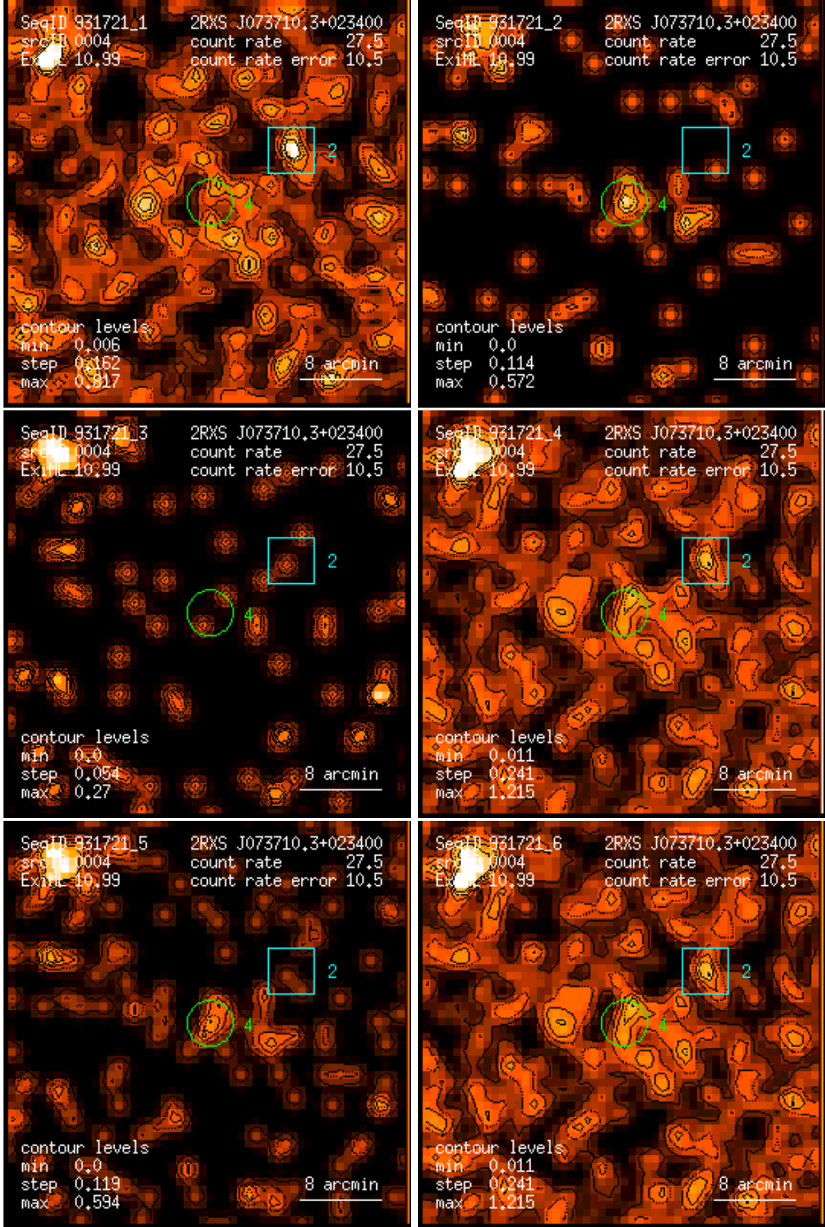
Figure 4: RASS 931721: detection 0004: band rate images, Gaussian filter: (1) PSPC channels 11 – 41, (2) 52 – 90, (3) 91 – 201, (4) 11 – 235, (5) 52 – 201, (6) 11 – 201. Broad band rates in counts/ks. Band rate contour levels in counts/ks/arcmin 2 .
