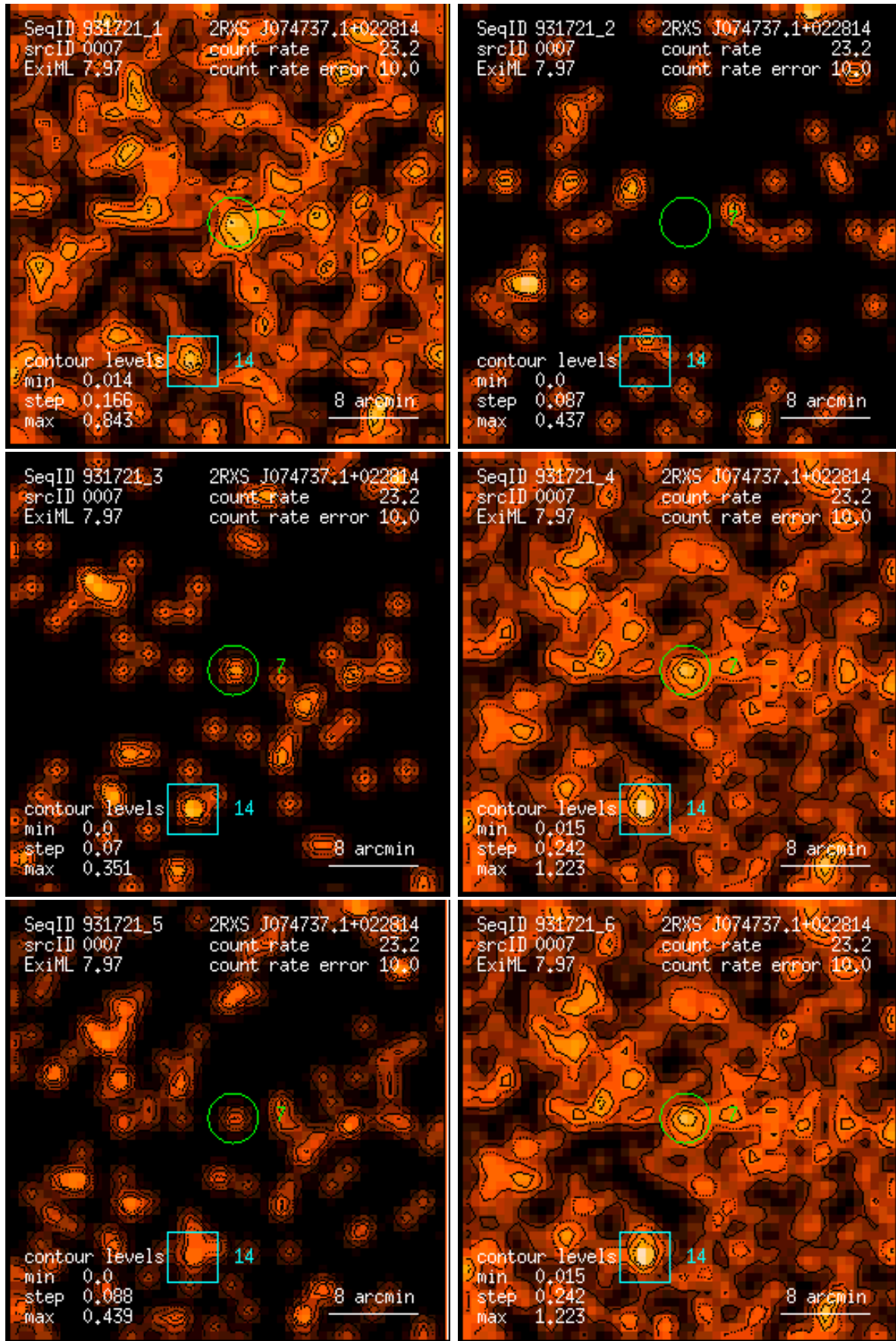
Figure 7: RASS 931721: detection 0007: band rate images, Gaussian filter: (1) PSPC channels 11 – 41, (2) 52 – 90, (3) 91 – 201, (4) 11 – 235, (5) 52 – 201, (6) 11 – 201. Broad band rates in counts/ks. Band rate contour levels in counts/ks/arcmin 2 .
