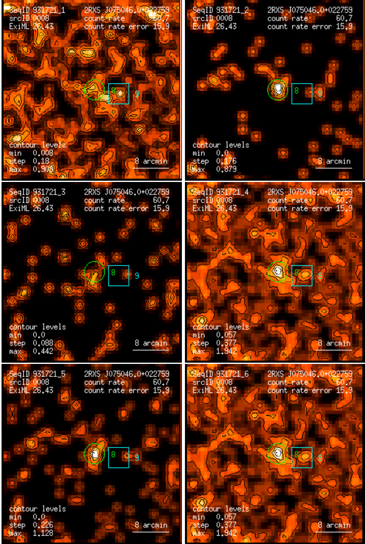
Figure 8: RASS 931721: detection 0008: band rate images, Gaussian filter: (1) PSPC channels 11 – 41, (2) 52 – 90, (3) 91 – 201, (4) 11 – 235, (5) 52 – 201, (6) 11 – 201. Broad band rates in counts/ks. Band rate contour levels in counts/ks/arcmin 2 .
