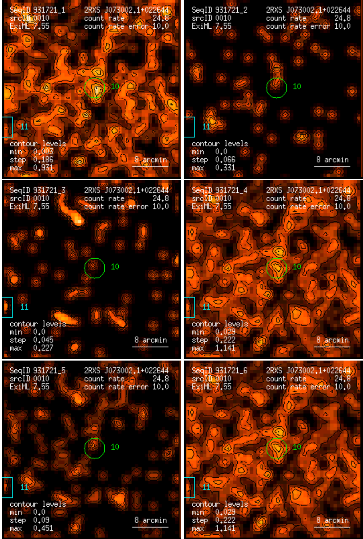
Figure 10: RASS 931721: detection 0010: band rate images, Gaussian filter: (1) PSPC channels 11 – 41, (2) 52 – 90, (3) 91 – 201, (4) 11 – 235, (5) 52 – 201, (6) 11 – 201. Broad band rates in counts/ks. Band rate contour levels in counts/ks/arcmin 2 .
