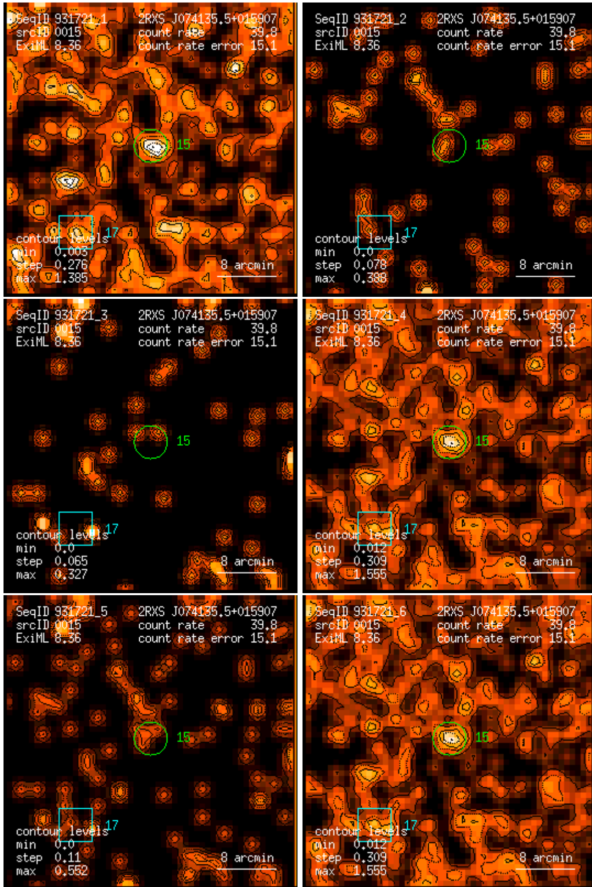
Figure 15: RASS 931721: detection 0015: band rate images, Gaussian filter: (1) PSPC channels 11 – 41, (2) 52 – 90, (3) 91 – 201, (4) 11 – 235, (5) 52 – 201, (6) 11 – 201. Broad band rates in counts/ks. Band rate contour levels in counts/ks/arcmin 2 .
